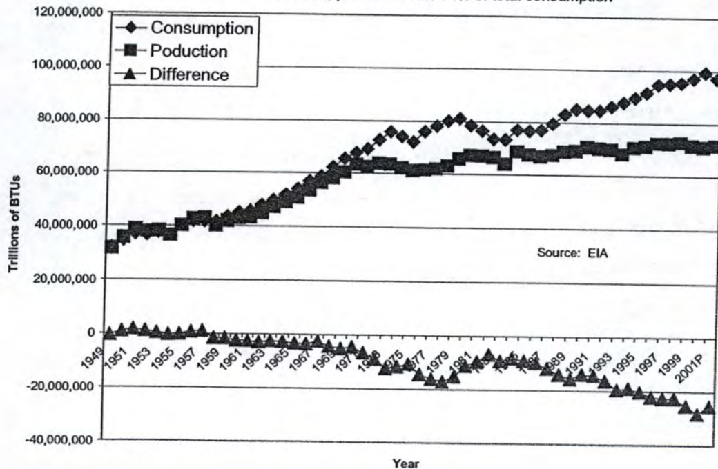
U.S. Energy Consumption/Production GAP 1949-2001
