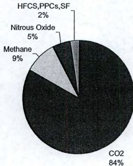
Composition of US Greenhouse Gasses 2000 Total Man-Made Greenhouse Gasses-- 1,906 Metric Tons of Carbon Equivalent
