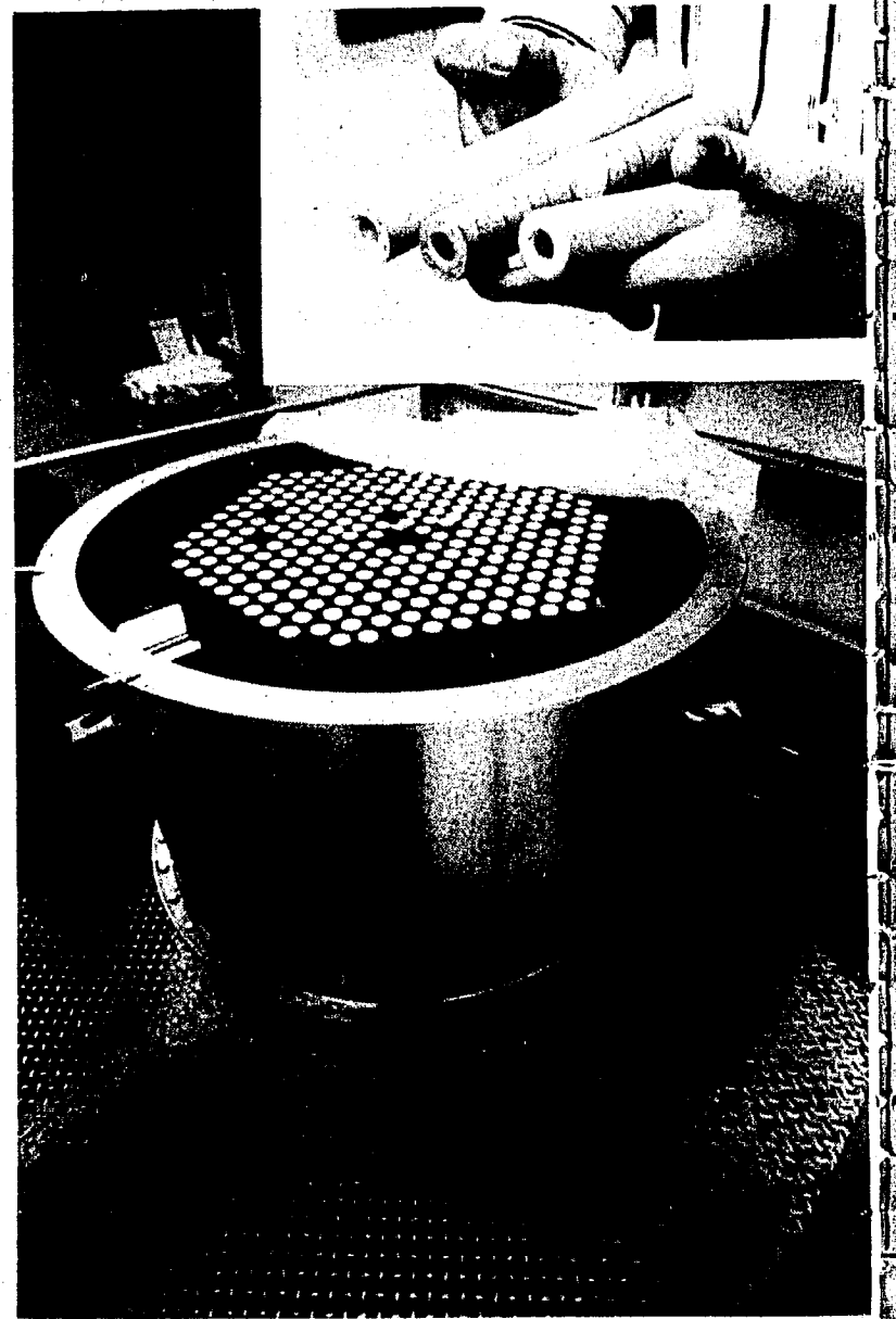
The inner workings of the U of I research nuclear reactor can be clearly seen when the plastic Tarpaulin cover is drawn back. The rods in the center of the tank contain some 4000 pounds of uranium in the same form as three fuel rods held by Kris Smith, university radiation officer (inset). Photo by Bob Bain.
