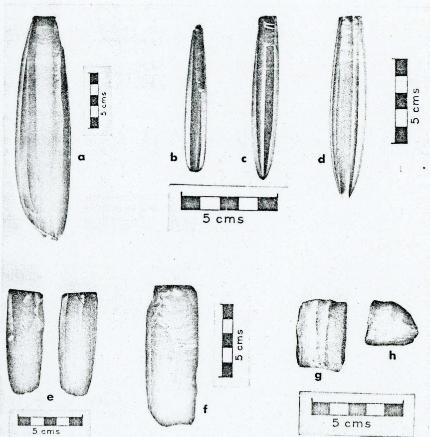
FIG. 1. Aboriginal cores. a, large obsidian polyhedral core from Colima, Mexico (I.S.U.M. Cr 1076); b, obsidian polyhedral core from Puebla, Mexico (I.S.U.M. Cr 1077); c, obsidian polyhedral core from Taxco, Mexico, (I.S.U.M. Cr 1079; notice on b and c the step fractures [angular breaks] from last attempts to detach blades); d, obsidian polyhedral core from Teotihuacán, Mexico (I.S.U.M. Cr. 1078; note the perfect termination of all blade scars); e, (I.S.U.M. Cr 1081) and f, (I.S.U.M. Cr 1080) obsidian cores from Teotihuacán, Mexico, showing blade removal on one side and original cortex surface on the other side of the core; g, blade surface (negative scars of previously detached blades) and h, platform surface of a small rectangular Hopewellian blade core from Ohio (I.S.U.M. Cr 1167).
