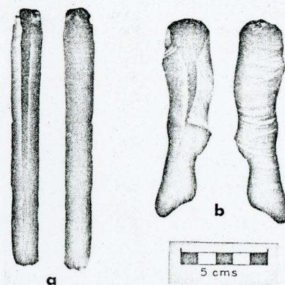
Fig. 7. Comparison of obsidian blades made by pressure and indirect percussion techniques. Both specimens produced by Crabtree. a , shows front and back surfaces of an obsidian blade made by pressure (I.S.U.M. Cr 1180); b , shows front and back surfaces of an obsidian blade made by indirect percussion (I.S.U.M. Cr 1182; notice the straight nearly parallel edges of a , the irregularity of the edges of b , and the heavy undulations and the prominent bulb of force on the back surface of b , which are much more subdued on a ).
