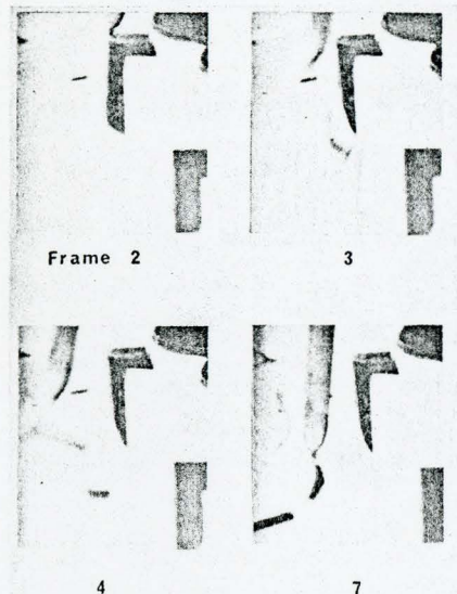
Fig. 14. Series of high-speed photographs, taken at 5,000 frames per second, showing removal of the distal end of the core. Frame 2—The core is placed in the clamp with the crutch tip positioned on the platform and downward pressure being applied. Frame 3—The blade has been detached from the core and appears as a blur just to the left of and slightly below the core. Note the change of position of the core in the clamp and the change of shape of the face of the core. The core was not properly secured in the clamp, and, when outward pressure was applied, the core tipped outward changing the angle of applied force resulting in excessive downward pressure and removal of the distal end of the core. Frame 4—The blade has broken and appears as two blurs below the crutch tip and to the left of and beneath the core. Frame 7—The two blade fragments are resting on the floor. The fragment just beneath the crutch tip is the distal end of the blade, the shape and heaviness of this portion showing that the distal end of the core has been removed. Compare the path of travel of the crutch tip in this series with the movements of the crutch tip in Figs. 11, 12, and 13.
