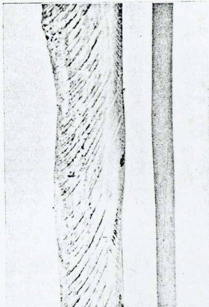
Fig. 10. Portion of the back surface of a large prismatic blade of glass (I.S.U.M. Cr 1141) produced by Crabtree, by pressure, showing the characteristic striations or fissures. Note the regularity of spacing of the fissures and the direction they point, indicating the direction from which force was applied to remove the blade. The platform or proximal end of the blade is beyond the upper margin of the picture.
