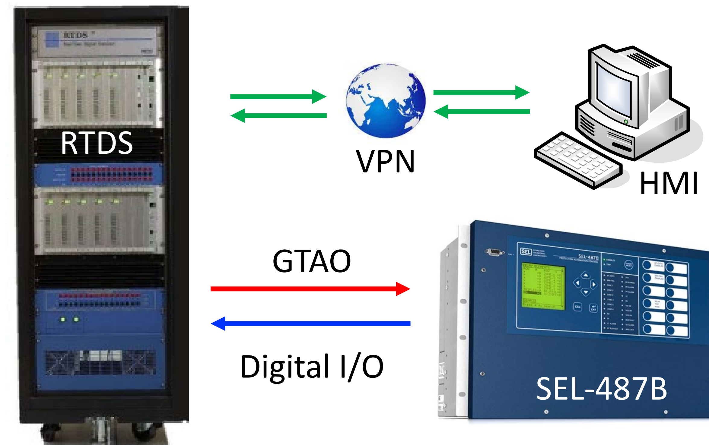
Communications Diagram
