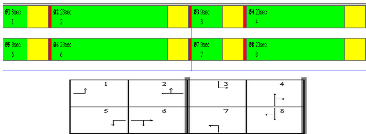
Figure 13 Synchro timings and a NEMA standard phasing
