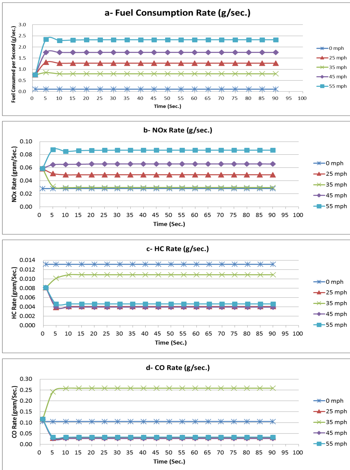
Figure 8 Fuel consumption and emission rates for the cases of idling and cruising
