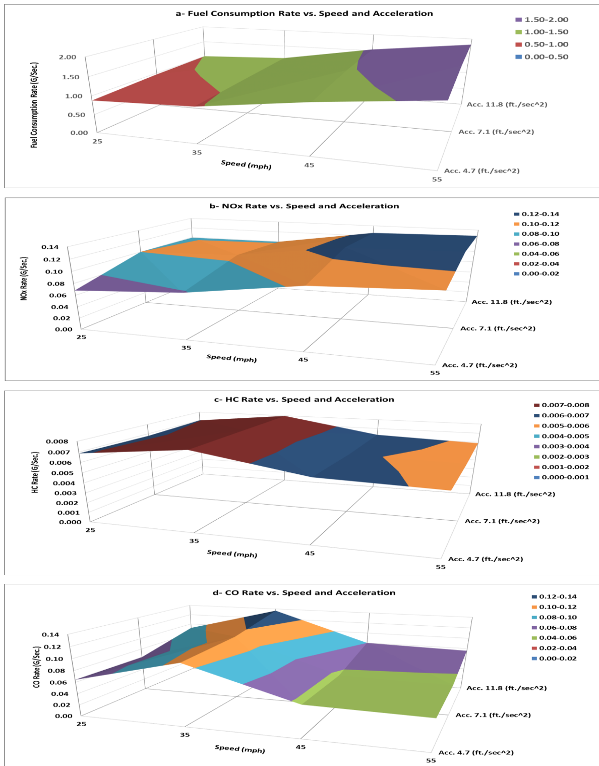
Figure 10 Fuel consumption and emission rates for the cases of accelerating from zero to 55 mph using different acceleration values (gram/sec.)
