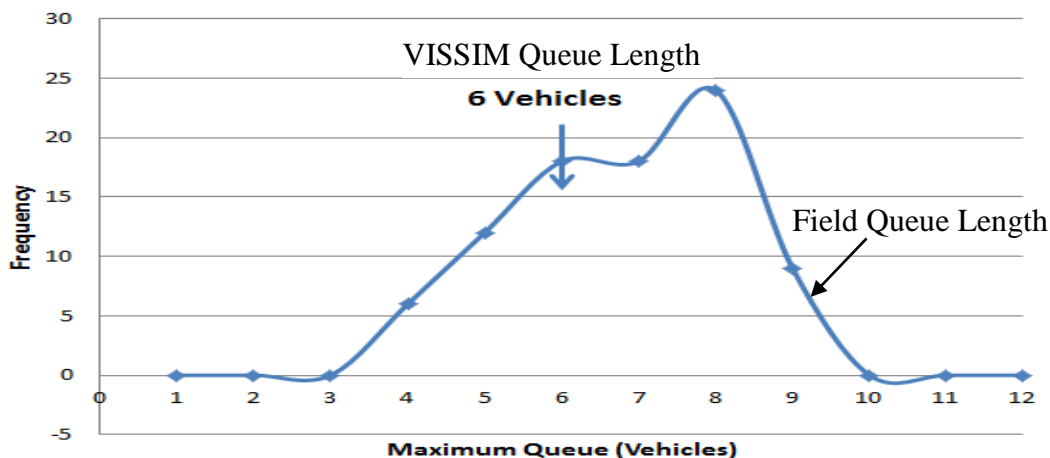
Figure 12 VISSIM vs. Field queue distribution in the SB direction of US95
