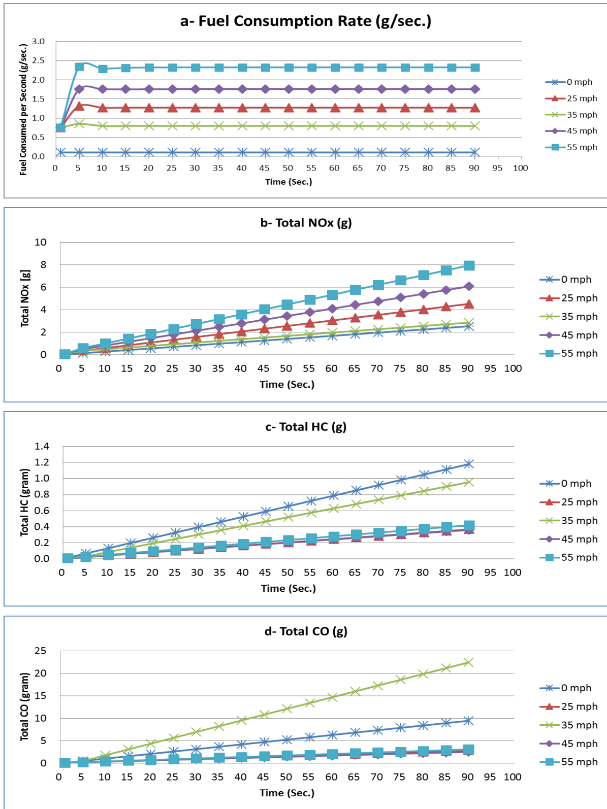
Figure 9 Total Fuel consumption and emissions for the cases of idling and cruising
