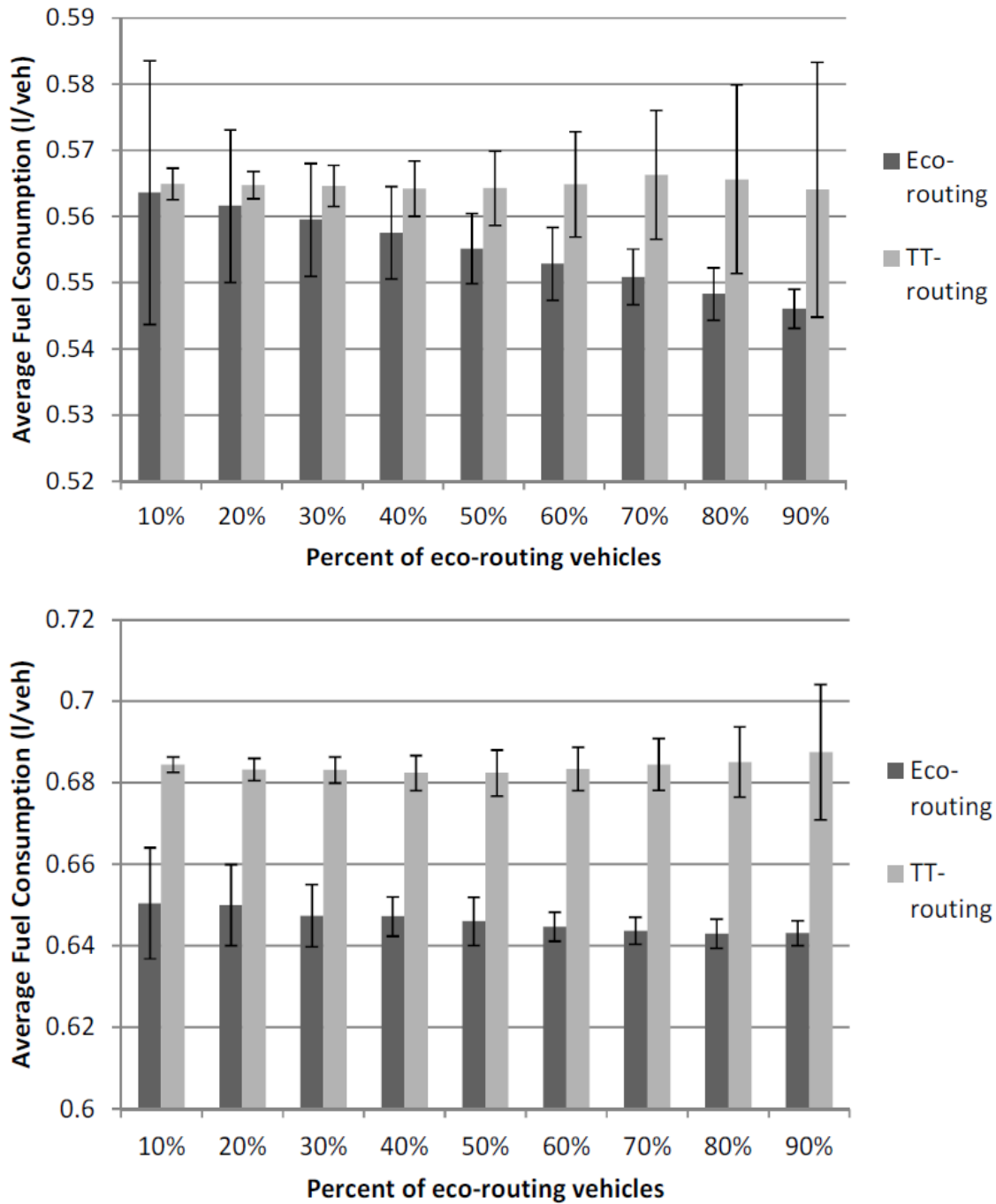
Figure 1 ECO-routing market penetration impact on network-wide fuel consumption levels versus minimum travel time (TT) routing
