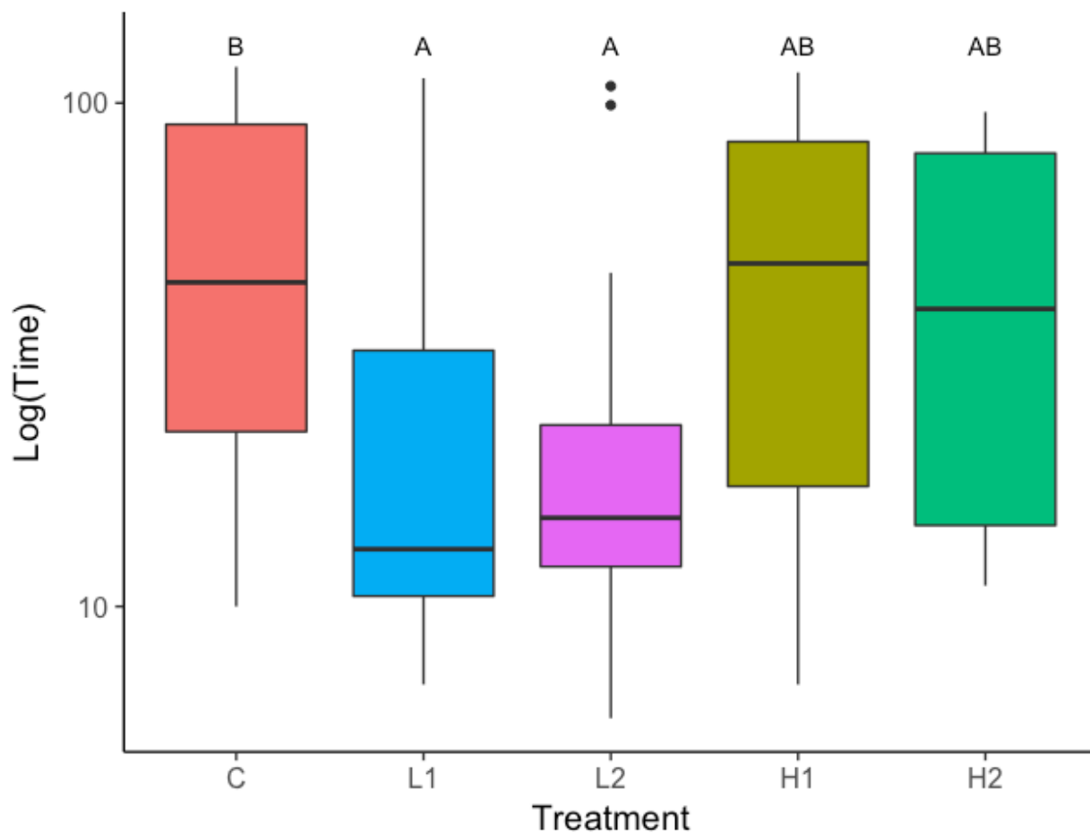
Figure 1.11. Passage times (log transformed) of a vertical slot weir in an experimental flume by treatment level, 2018. Median passage times for each treatment are as follows: C=44.5 min, L1=13 min, L2=15 min, H1=48 min, H2 = 39 min. Boxes with different letters indicate significant differences between treatments. Treatment factors refer to the following: C= control; L1 = low velocity, low duration; L2 = low velocity, high duration; H1 = high velocity, low duration; H2 = high velocity, high duration.
