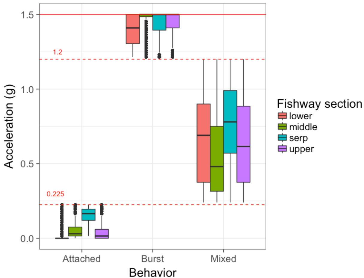
Figure 2.6. Distribution of all acceleration (g) records by each behavior within each fishway section for all fish (n=44). Red dashed line indicates threshold for attached and mixed behavior categories. Red solid line indicates upper threshold for burst behavior category.
