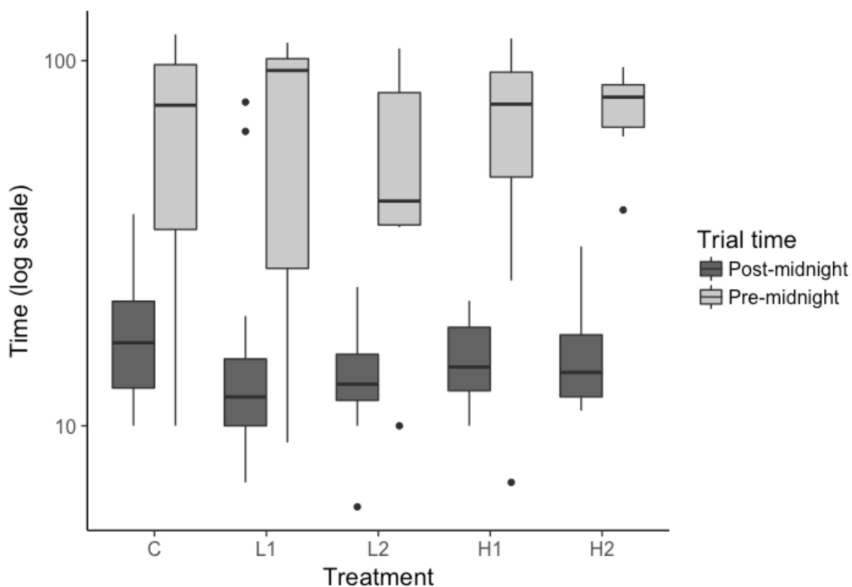
Figure 1.12. Passage times (log transformed) of a vertical slot weir in an experimental flume by treatment level and trial time, 2018. Median passage times of pre-midnight trials are as follows: C=75.5 min, L1=94 min, L2=41.5 min, H1=76 min, H2=79.5 min versus median passage times of post-midnight trials C=17 min, L1=12 min, L2=13 min, H1=14.5 min, H2=14 min. Treatment factors refer to the following: C= control; L1 = low velocity, low duration; L2 = low velocity, high duration; H1 = high velocity, low duration; H2 = high velocity, high duration.
