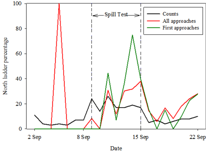
Figure 2. Daily percent use of the north fishway at The Dalles Dam by adult steelhead based on ladder-specific counts (of steelhead only) and of total fishway approaches and first fishway approaches by unique, radio-tagged steelhead in September 2014 before, during, and after the spill test. Note that sample sizes were low (<10) during the pre-spill period.
