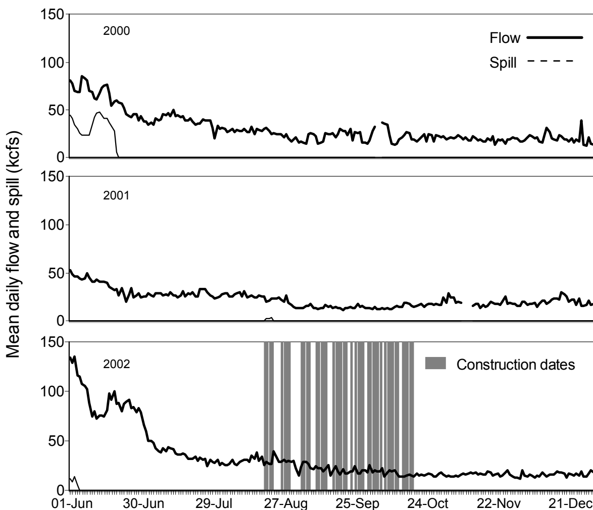
Figure 2. Mean daily flow and spillway discharge at Lower Monumental Dam from 1 June to 31 December 2000, 2001, and 2002.
