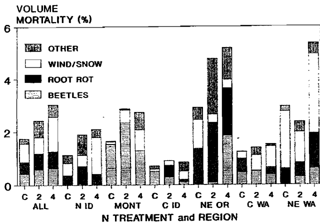
Figure 3. Average Douglas-fir mortality rates (% of total volume) by geographic region, nitrogen fertilizer treatment, and cause of mortality for the six years following fertilization. Fertilizer treatments are 0 (C), 224 (2), and 448 (4) kg N/ha. Modified from Mika and Vanderploeg (1991).
