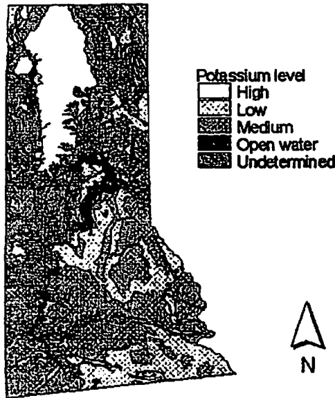
Figure 6. Rock potassium content map for the five northern Idaho counties.
