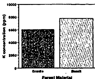
Figure 5. Foliar potassium concentration for unfertilized Douglas-fir stands growing on granite and basalt parent materials.
