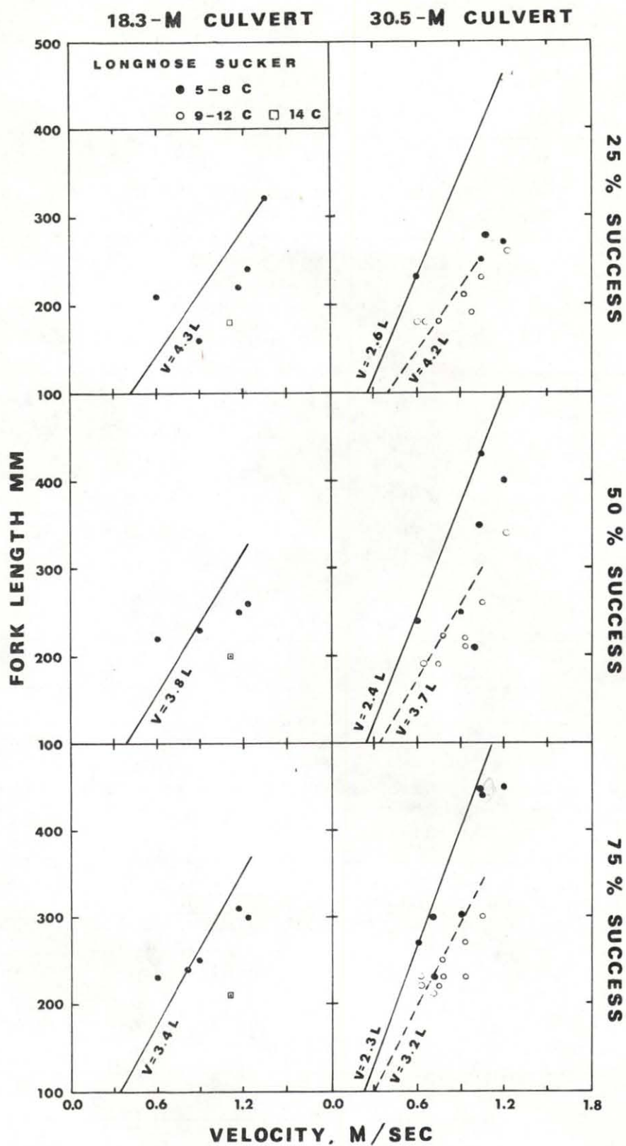
Fig. 17. Relationship between fork lengths and water velocities which permitted 25, 50 and 75 percent of the longnose suckers to ascend 18.3 and 30.5 m culverts in 1-day tests. Solid lines (5-8 C) and dashed lines (9-12 C) represent maximum "safe" velocities.
