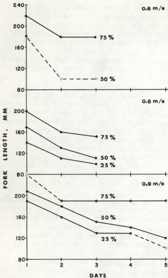
Fig. 19. Cumulative effect of time on the length of grayling that ascended a 30.5 m culvert at the indicated percentage level of success. Hollow points and dashed lines indicate extrapolated data.
