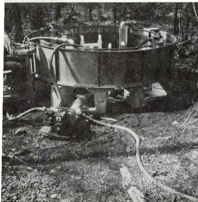
Fig. 21. View of circular swimming channel with installed pumps and hoses.
