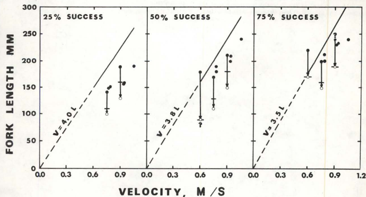
Fig.18. Effect of water velocity on the capability of grayling to ascend a 30.5 m culvert in 1-, 2- and 3-day trials (temperature, 9-16 C). Arrows indicate the direction of change of critical lengths for 3-day tests. Solid circle = 1-day test; cross bar = 2-day test; open circle = 3-day test; and a ? = extrapolated value to the next length class.
