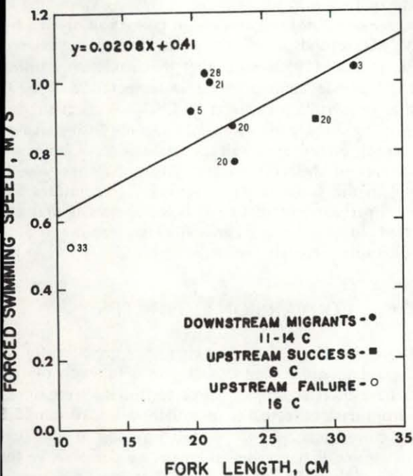
Fig. 26. Swimming speed of Arctic grayling compelled by a wire screen to swim at a constant rate for 1 hour in a circular flume. The numerals beside the points refer to the number of fish in a sample.
