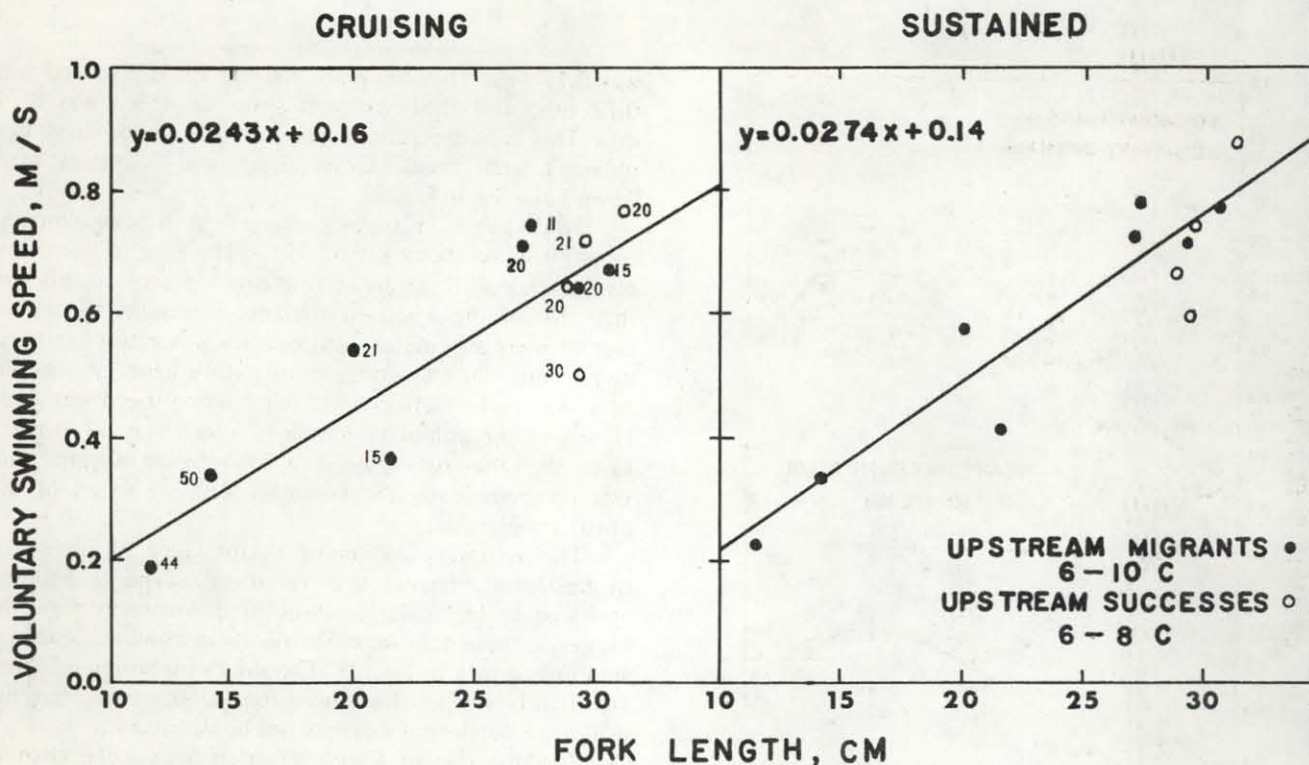
Fig. 24. Cruising and sustained speeds of upstream migrating Arctic grayling tested in a circular flume. The mean speeds of fish (hollow points) that successfully passed upstream through an 18.3 m culvert at a flow of 1.3 m/s are compared with speeds of randomly selected upstream migrants (solid points). The numerals beside the points refer to the number of fish in a sample. The same lots of fish were used for cruising and sustained speeds.
