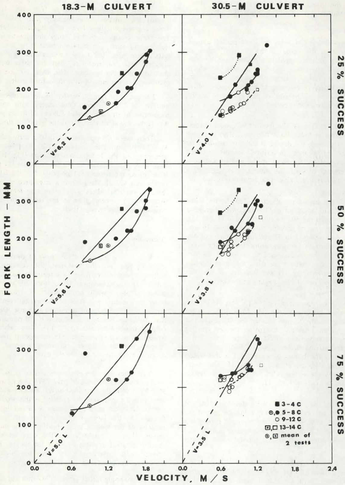
Fig. 16. Relationship between fork length and water velocities which permitted 25, 50 and 75 percent of Arctic grayling to ascend 18.3 and 30.5 m culverts in 1-day tests. Curved lines approximate "barrier" parameters (dotted, 3-4 C; solid, 5-8 C; dashed, 9-12 C). Straight lines represent maximum "safe" velocities.
