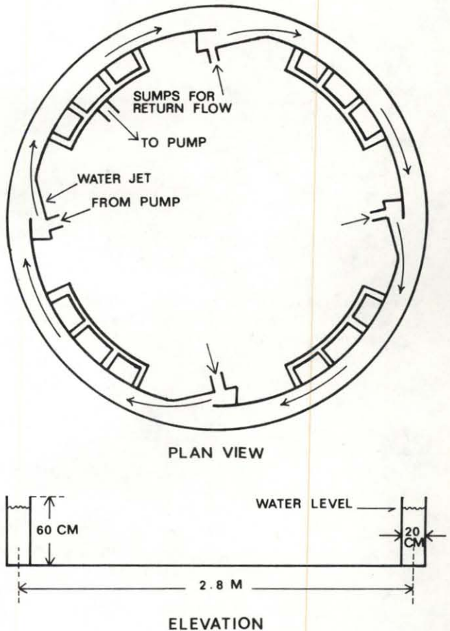
Fig. 20. Plan and elevation of circular channel used in fish swimming performance tests. Pumps and hoses are omitted from the diagram.
