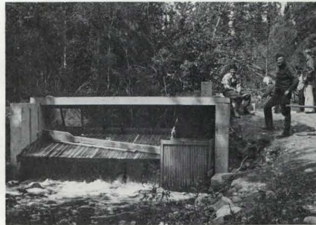
Fig. 5. View of dam with inclined plane trap installed for collection of downstream migrants (1974).
