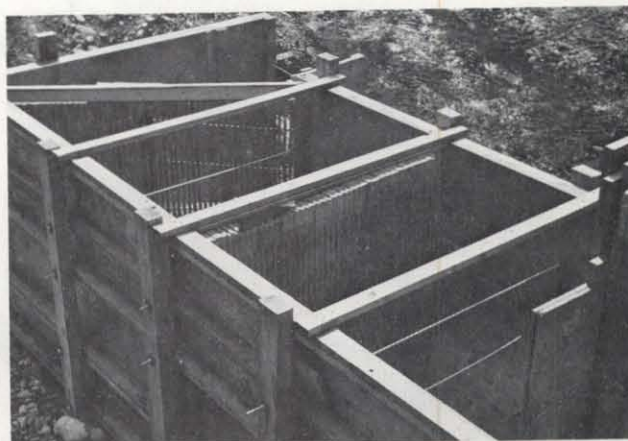
Fig. 15. Tailbox of the 30.5 m culvert facility showing the upstream experimental compartment (right) from which test fish could ascend the culvert and the downstream conditioning compartment (left) in which fish could recover overnight from any effects of netting.
