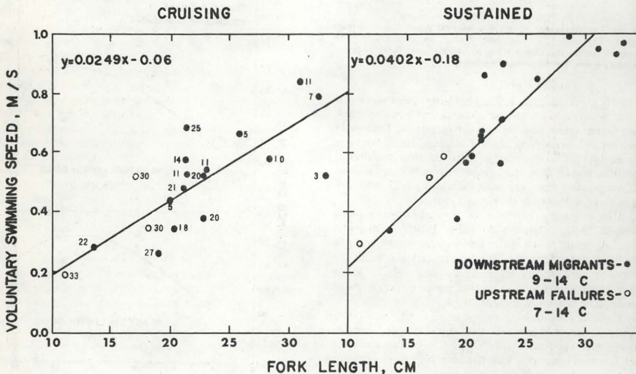
Fig. 25. Voluntary cruising and sustained speeds of downstream migrating Arctic grayling tested in a circular flume. The mean speeds of upstream migrants (hollow points) that failed to pass through an 18.3 m culvert at flows of 1.1, 1.5 and 1.6 m/s are compared with speeds of downstream migrants. The numerals beside the points refer to the number of fish in a sample. The same lots of fish were used for cruising and sustained speeds.
