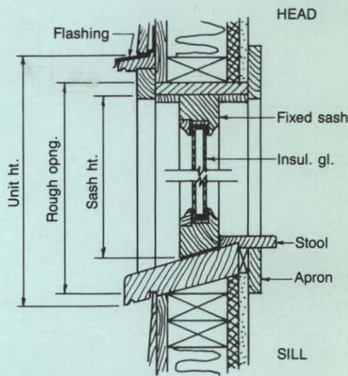
WINDOW SECTION
