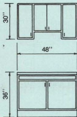
SINK UNIT WALL & BASE
