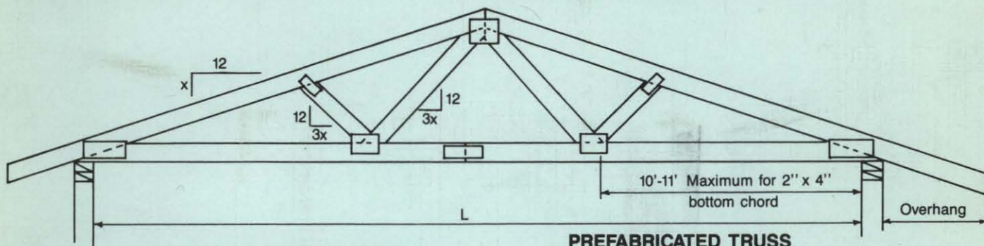
PREFABRICATED TRUSS
