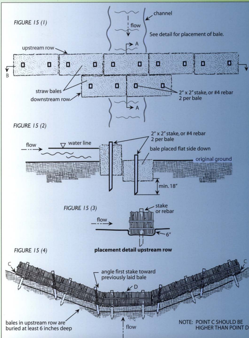
Figure 15. Straw bail check dams.
