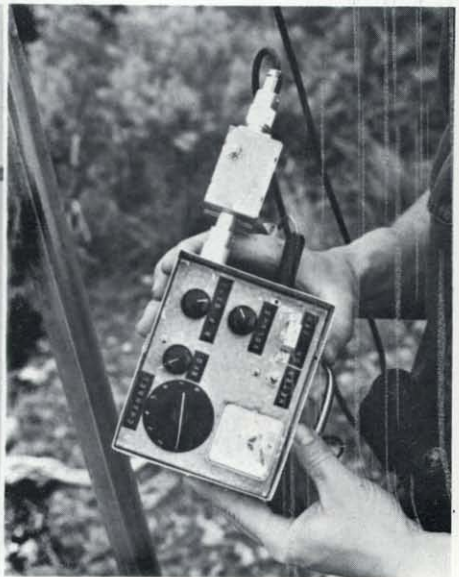
Figure 12. The 3-element yagi and the methods of attaching the amplifier and its power supply.
