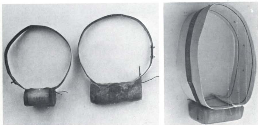
Figure 3. The fully assembled transmitters: A—Model 1 (30 MHz), B—Model 2 (30 MHz), and C—Model 3 (47 MHz).
