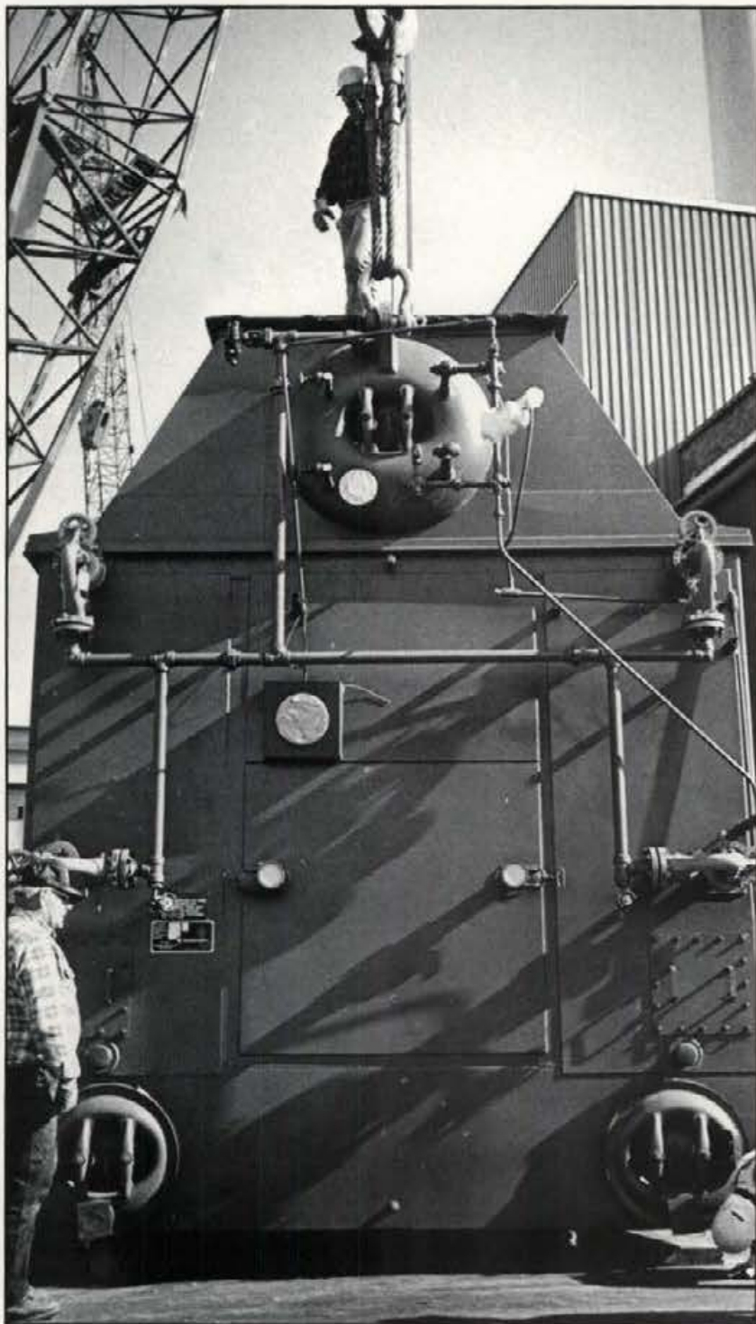
PORTIONS of Third, Line and Sixth streets were closed while two large cranes hoisted the new boiler into place behind the power plant. The boiler weighed nearly 180,000 pounds. (Hayes)
