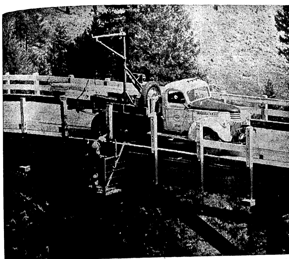
Photo shows bridge cage suspended over side of Plummer Creek bridge on Heyburn Park highway in Beneviah county. Cage was designed in state highway department's maintenance shop in Coeur d'Alene to facilitate repair and inspection work.
