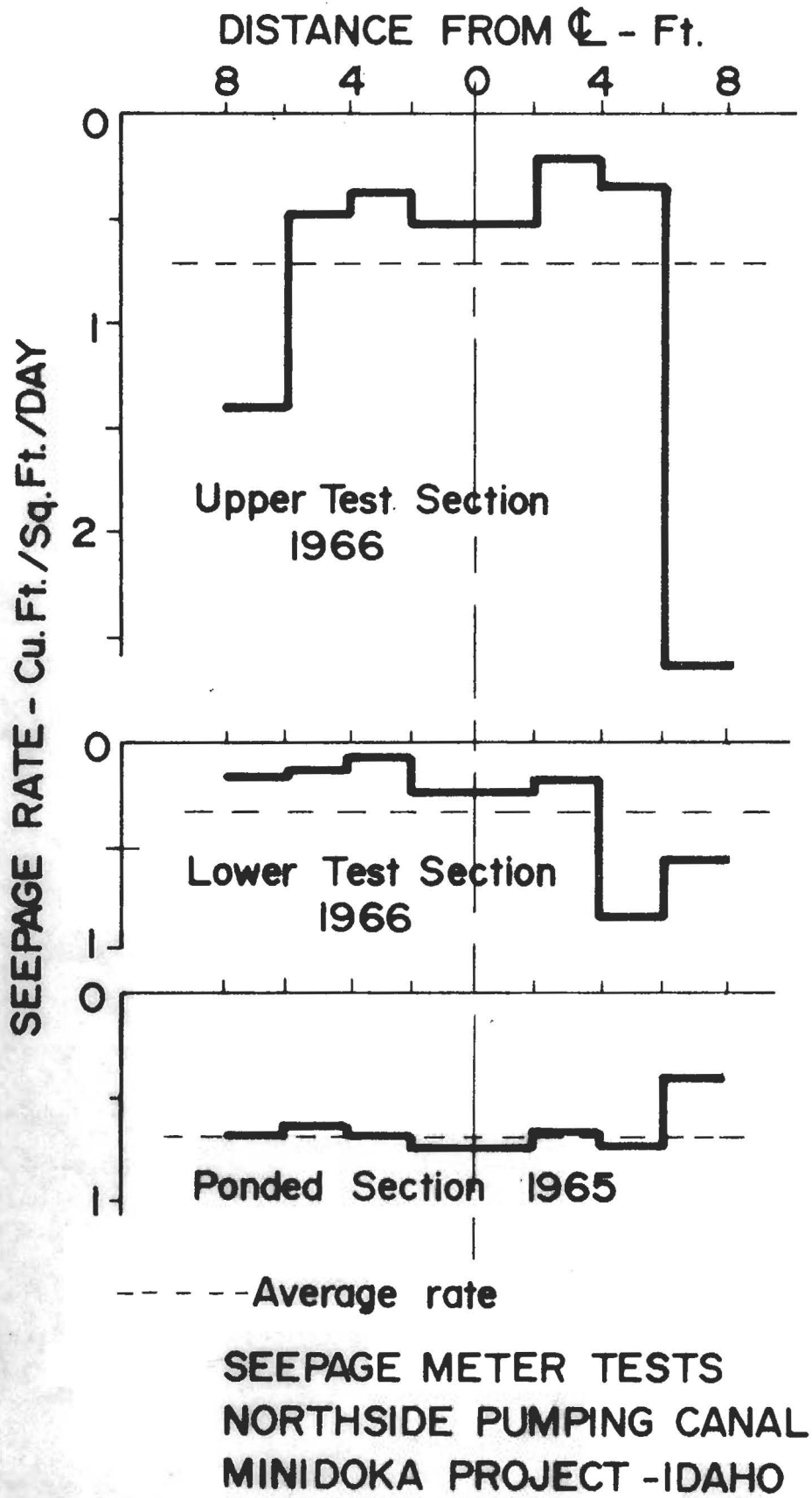
Figure 1. --Variation of seepage rate in cross-section.
