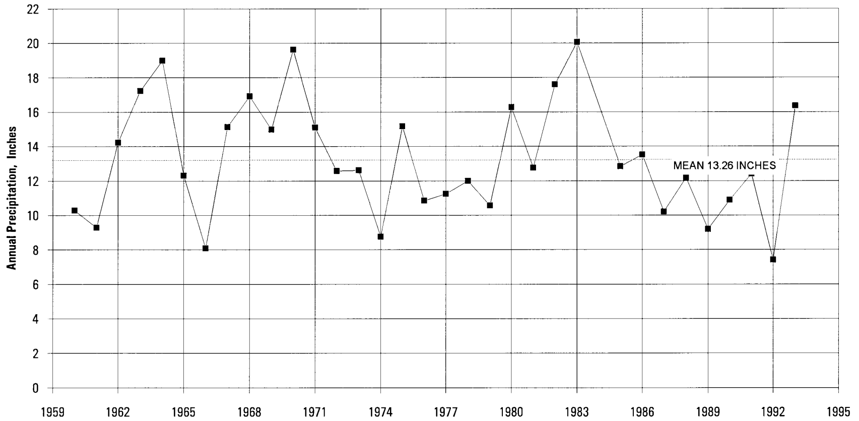
Figure 15. Annual Precipitation at Picabo Weather Station
