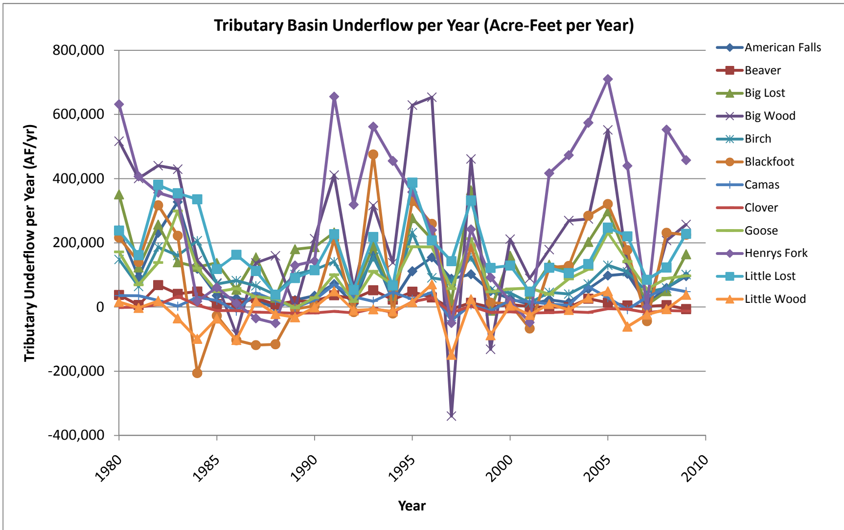
Figure 11a. Volumetric estimates of underflow for basins tributary to the Eastern Snake River Plain.
