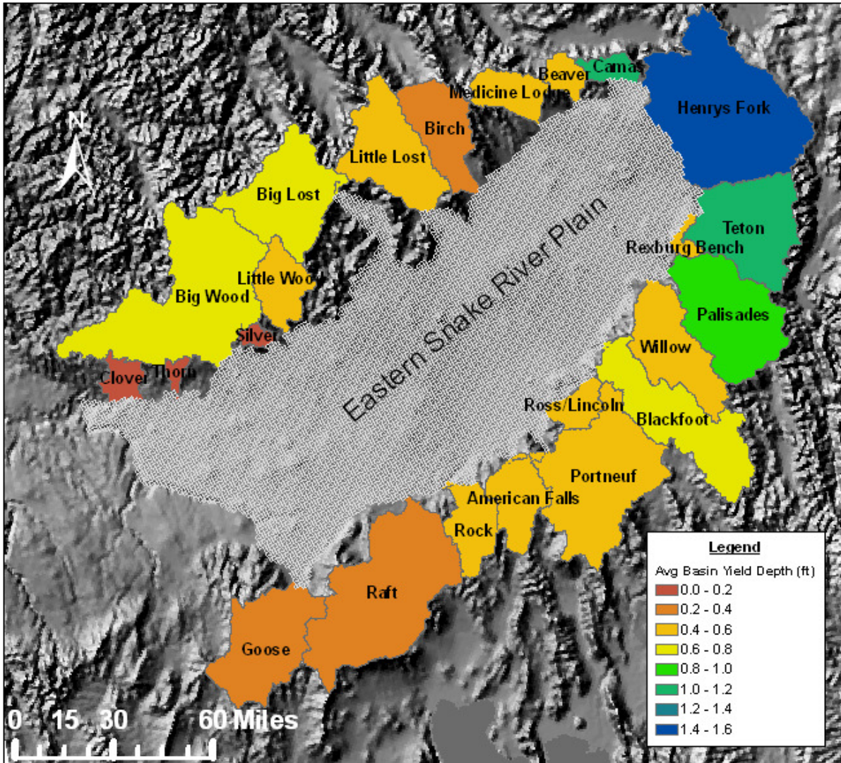
Figure 9. Average basin yield depths in feet for 1980 – 2009.
