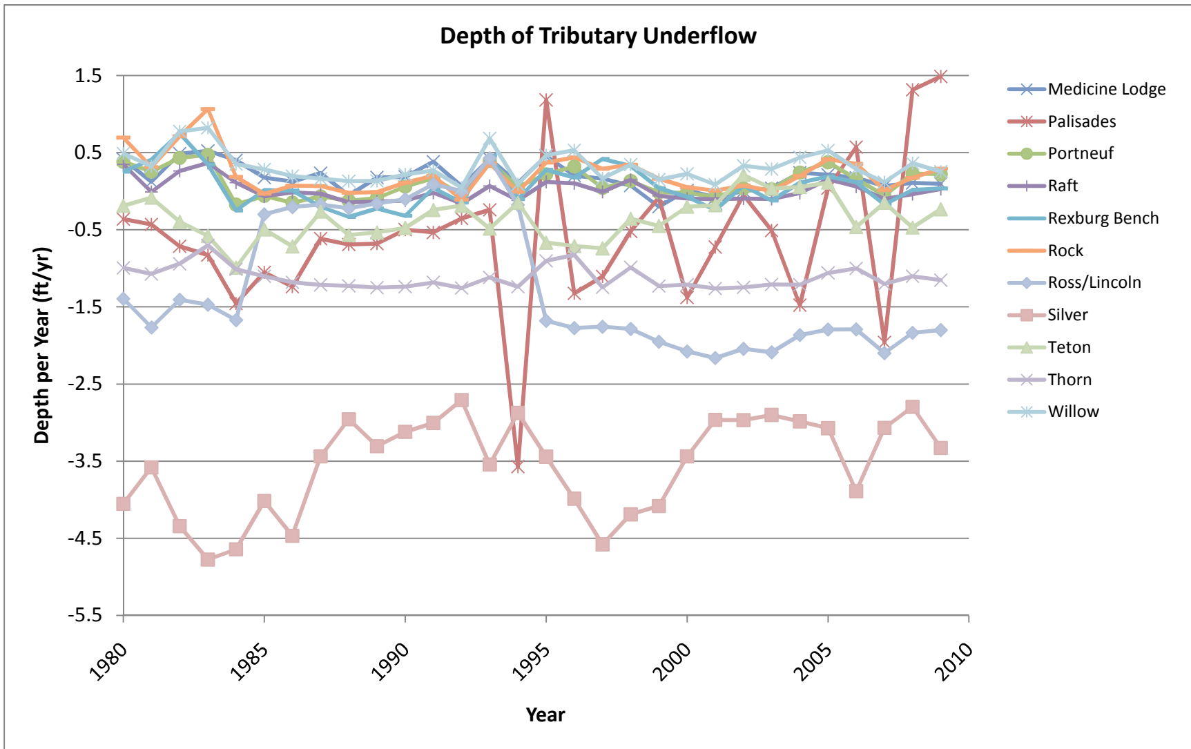
Figure 10b. Estimates of underflow as a depth for basins tributary to the Eastern Snake River Plain. Note that the vertical scale in this figure is different from Figure 10a.
