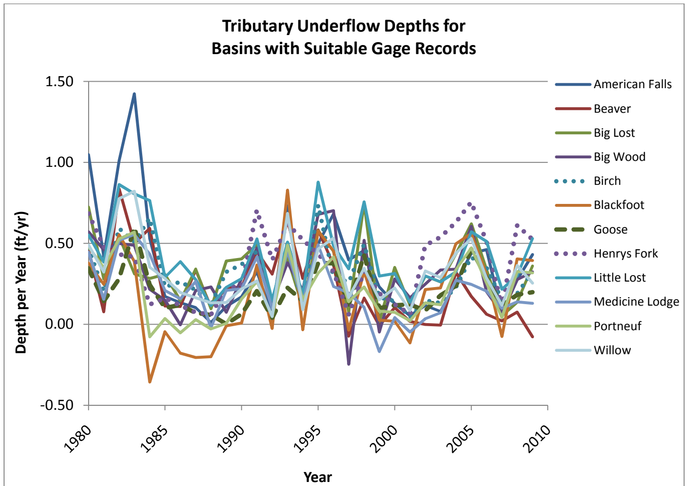
Figure 13. Tributary underflow depths for basins of the Eastern Snake Plain with suitable gage station records near the model boundary.
