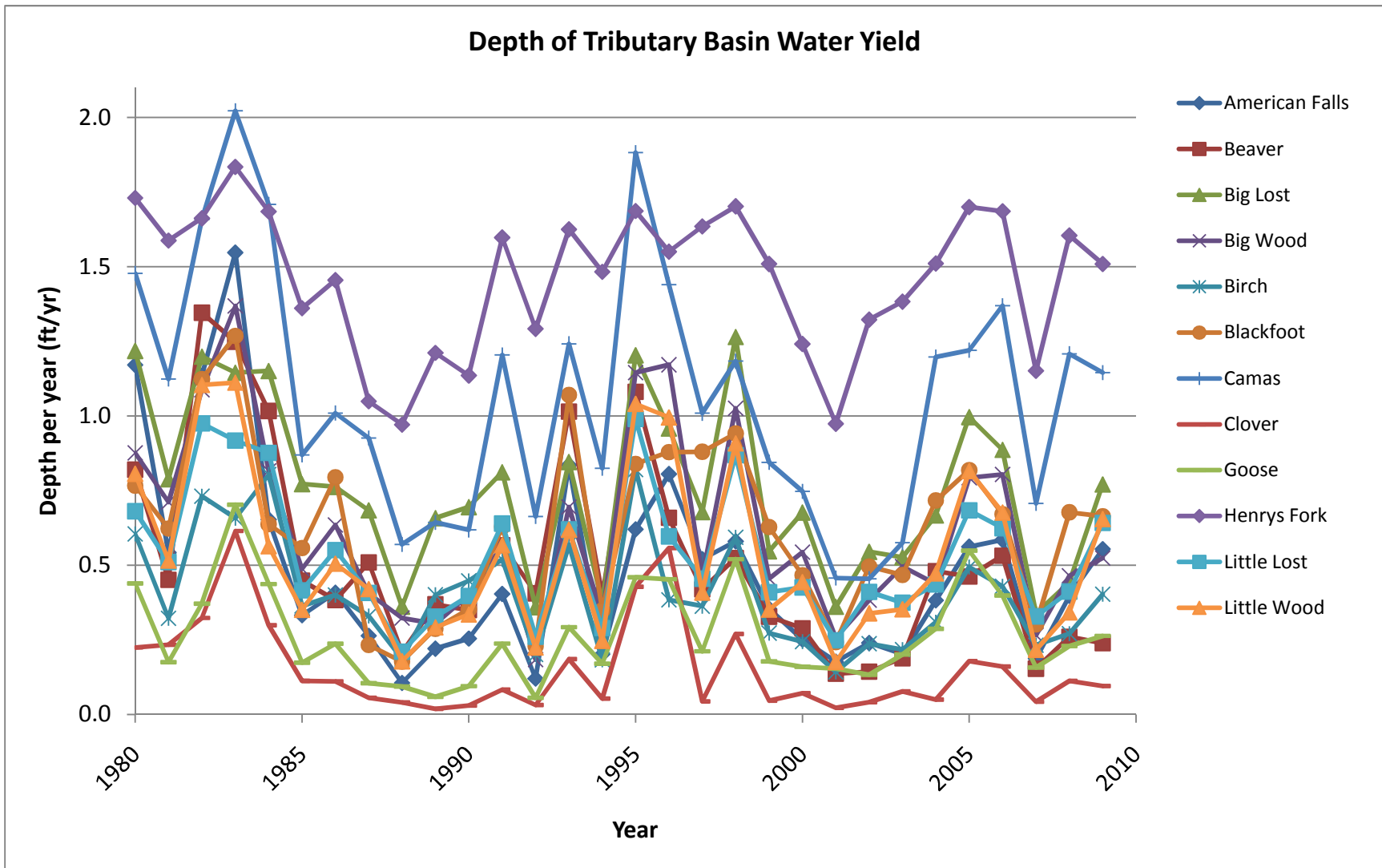
Figure 6a. Water yield depth for basins tributary to the Eastern Snake River Plain aquifer. Water yield calculated using the Langbein method (Nace et al. 1961).
