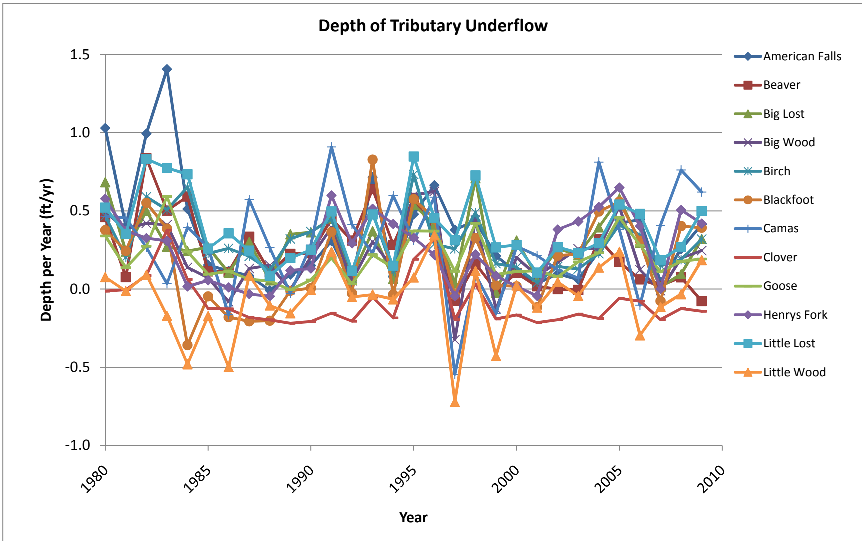
Figure 10a. Estimates of underflow as a depth for basins tributary to the Eastern Snake River Plain.
