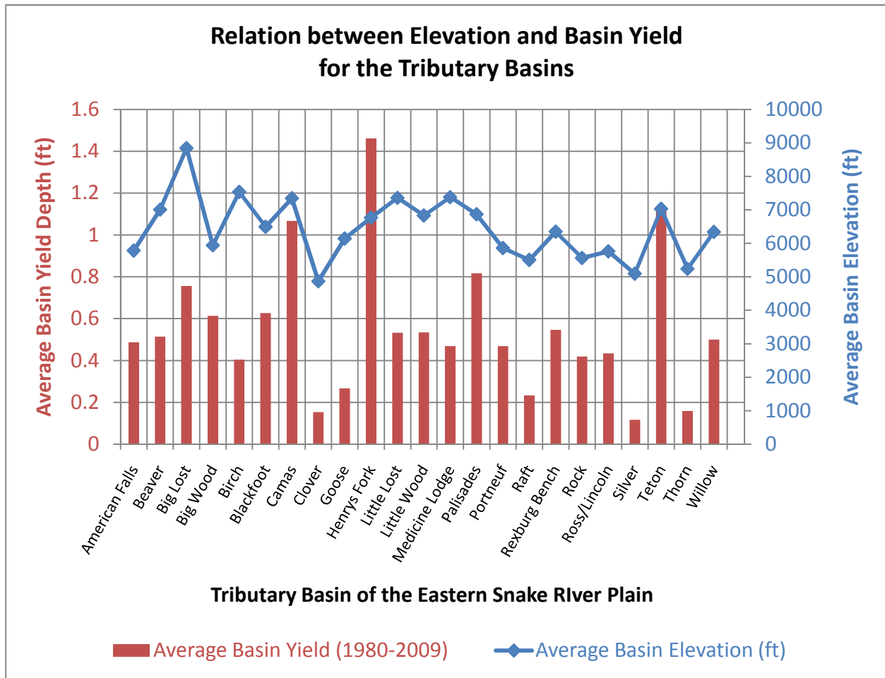
Figure 8. Tributary basin yield averages for 1980 - 2009.
