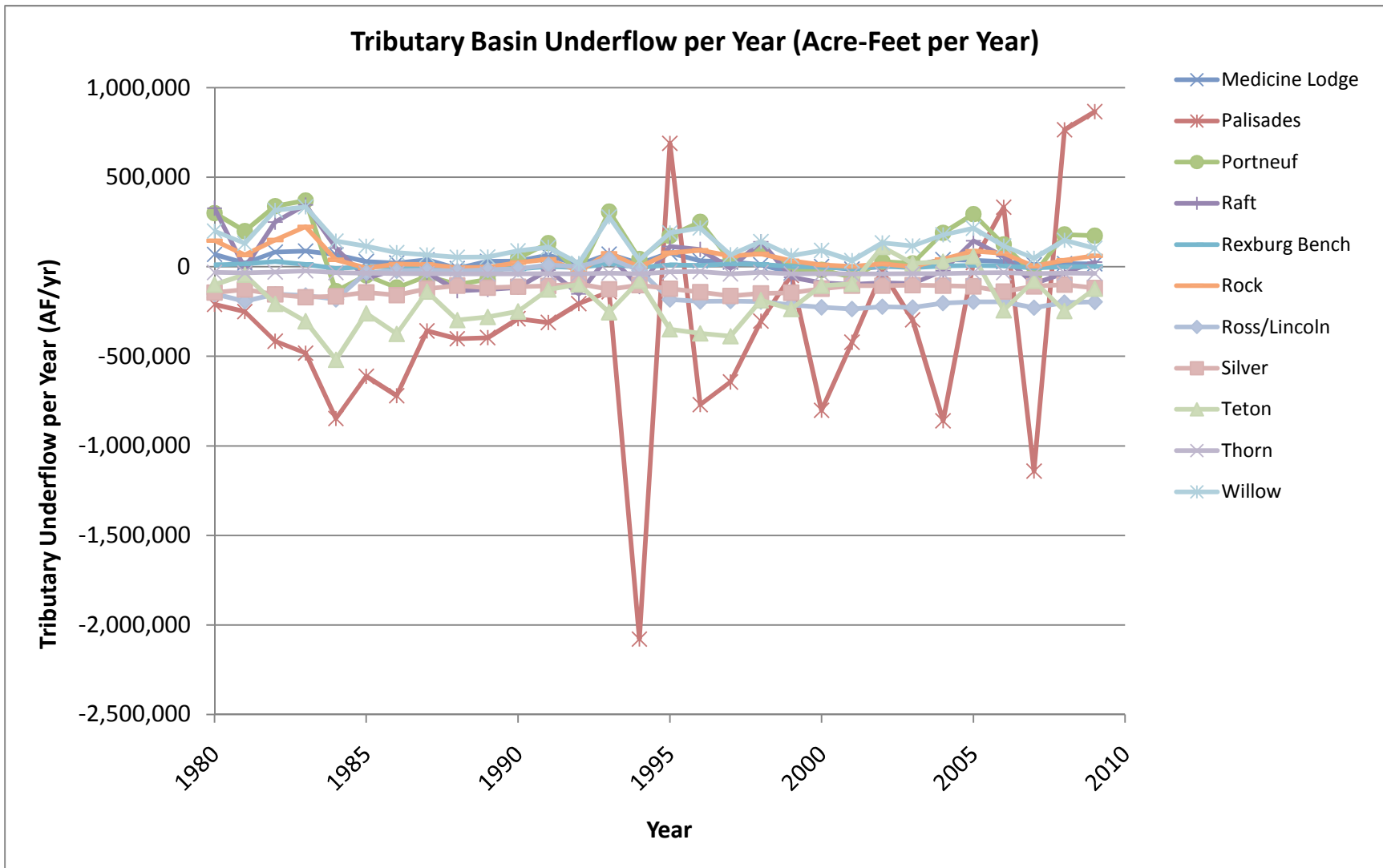
Figure 11b. Volumetric estimates of underflow for basins tributary to the Eastern Snake River Plain. Note that the vertical scale in Figure 11a is different than the scale in this figure.
