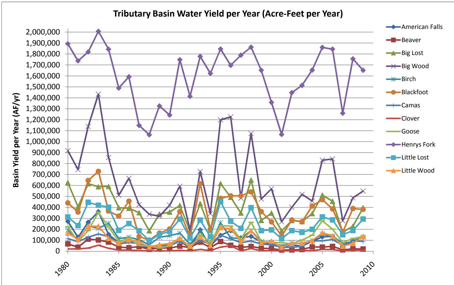
Figure 7a. Volume of water yield for tributary basins of the Eastern Snake River Plain aquifer. Water yield calculated using the Langbein method (Nace et al. 1961).
