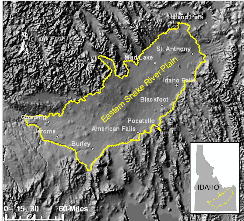
Figure 1. Eastern Snake River Plain Aquifer Boundary for the current aquifer model, ESPAM version 2.0.
