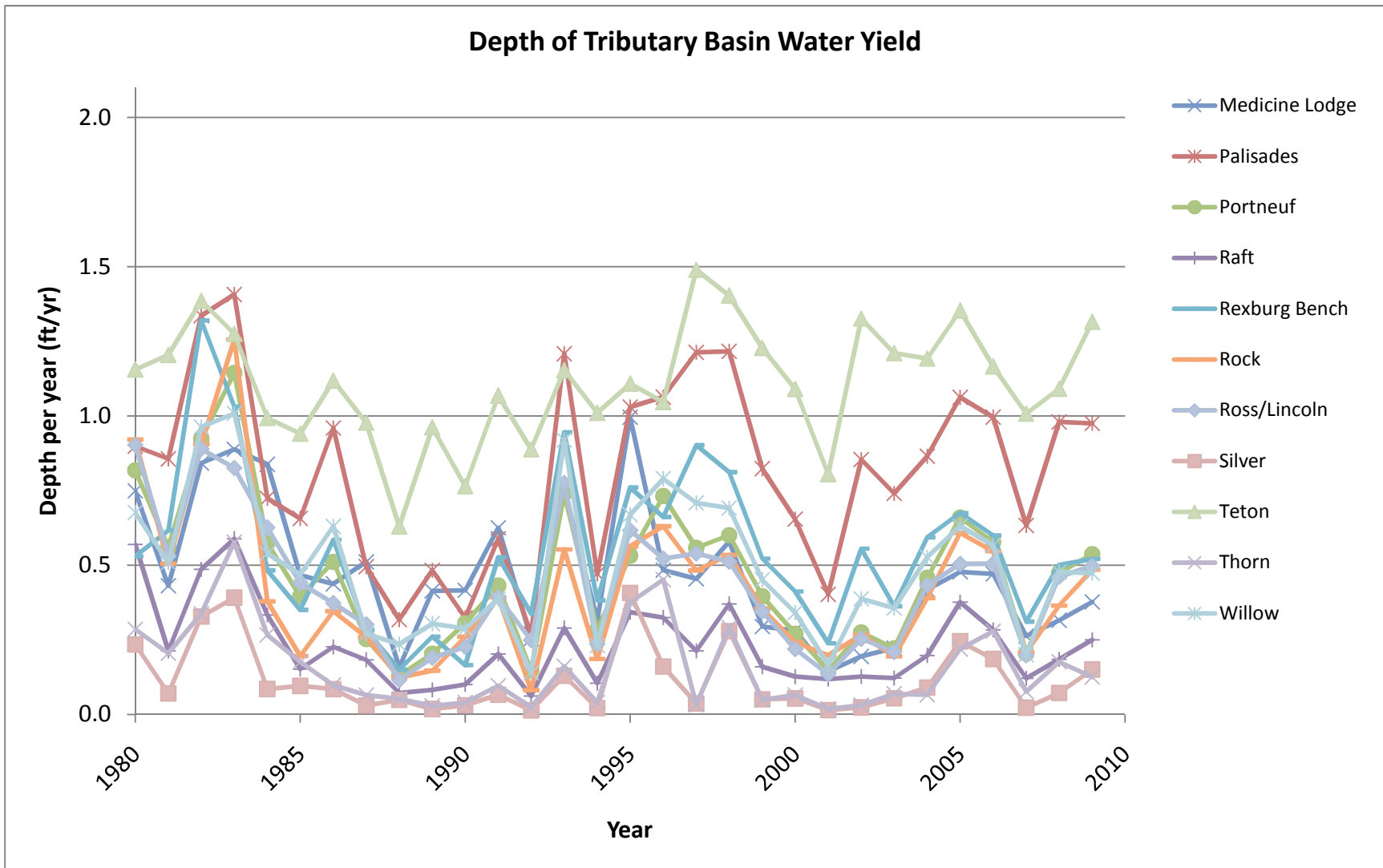
Figure 6b. Water yield depth for basins tributary to the Eastern Snake River Plain aquifer. Water yield calculated using the Langbein method (Nace et al. 1961).
