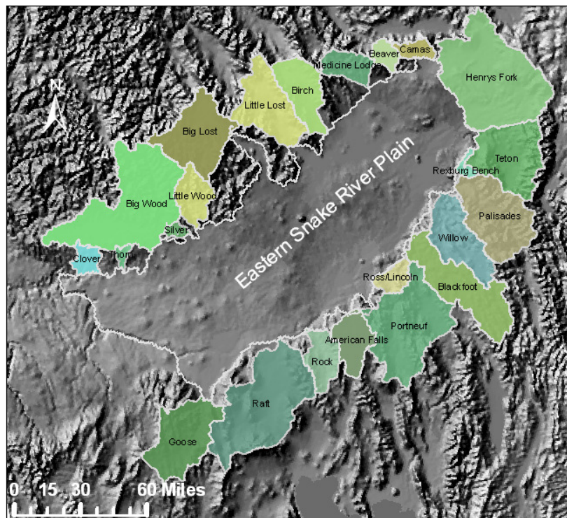
Figure 2. Tributary basin areas considered for estimating groundwater underflow.
