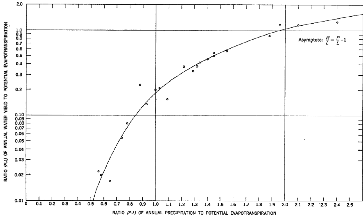
Figure 4. Relationship defined between annual water yield to precipitation and potential ET as defined by the Langbein method. Adapted from Figure 8, Nace et al. (1961).
