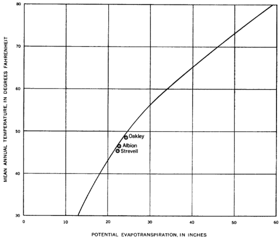
Figure 3. Defined curve between mean annual temperature and potential ET in North America. Adapted from Figure 7, Nace et al. (1961).
