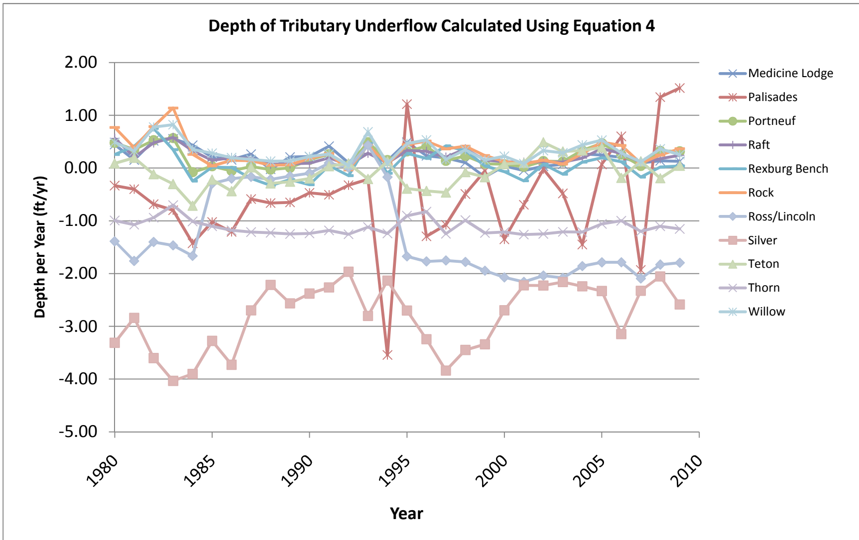
Figure 12b. Tributary underflow depths calculated using Equation 4. Note that this scale is different Figure 12a for the purpose of showing basins with larger values of depth.
