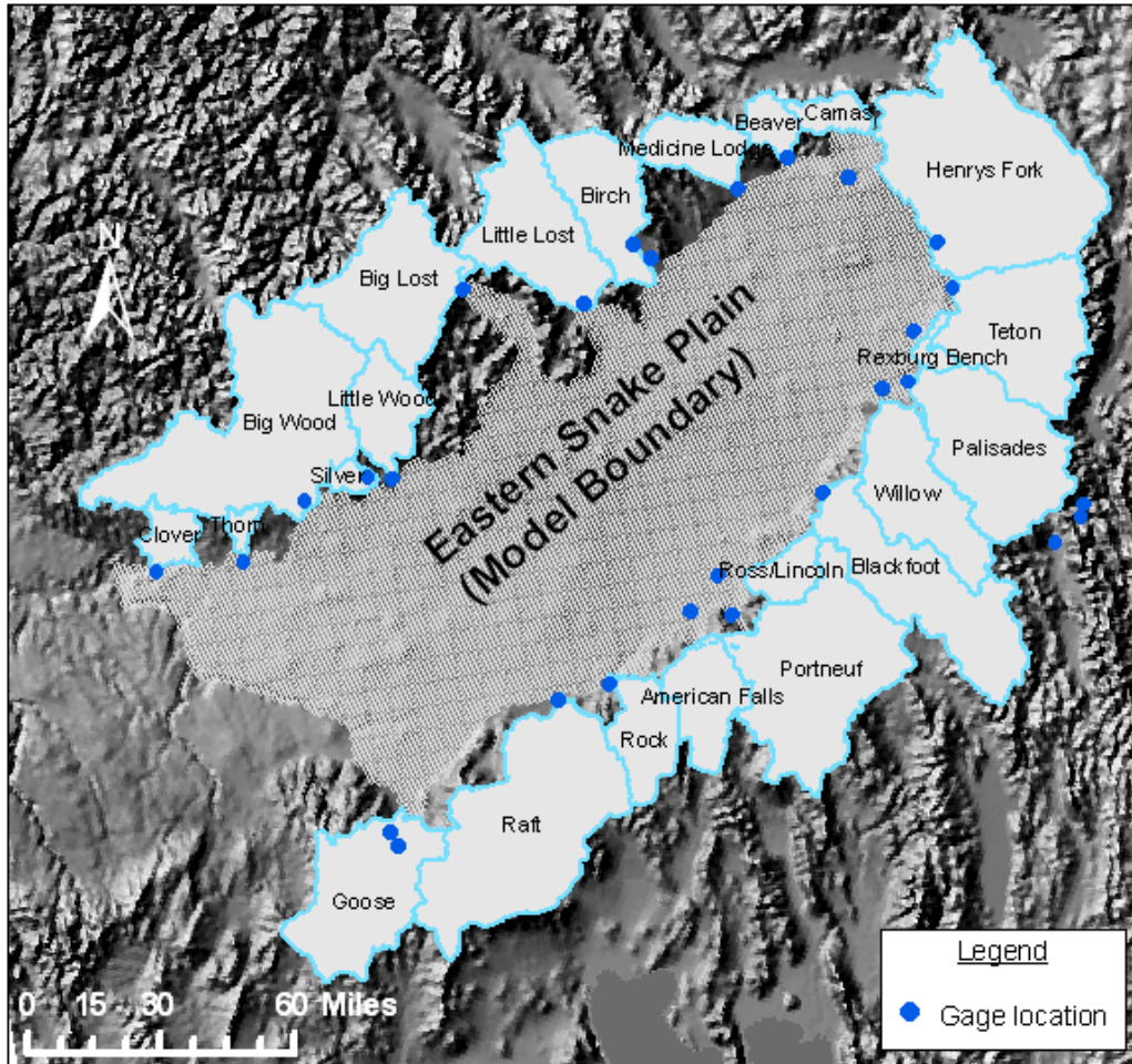
Figure 5. Gaged flow locations near the model boundary.
