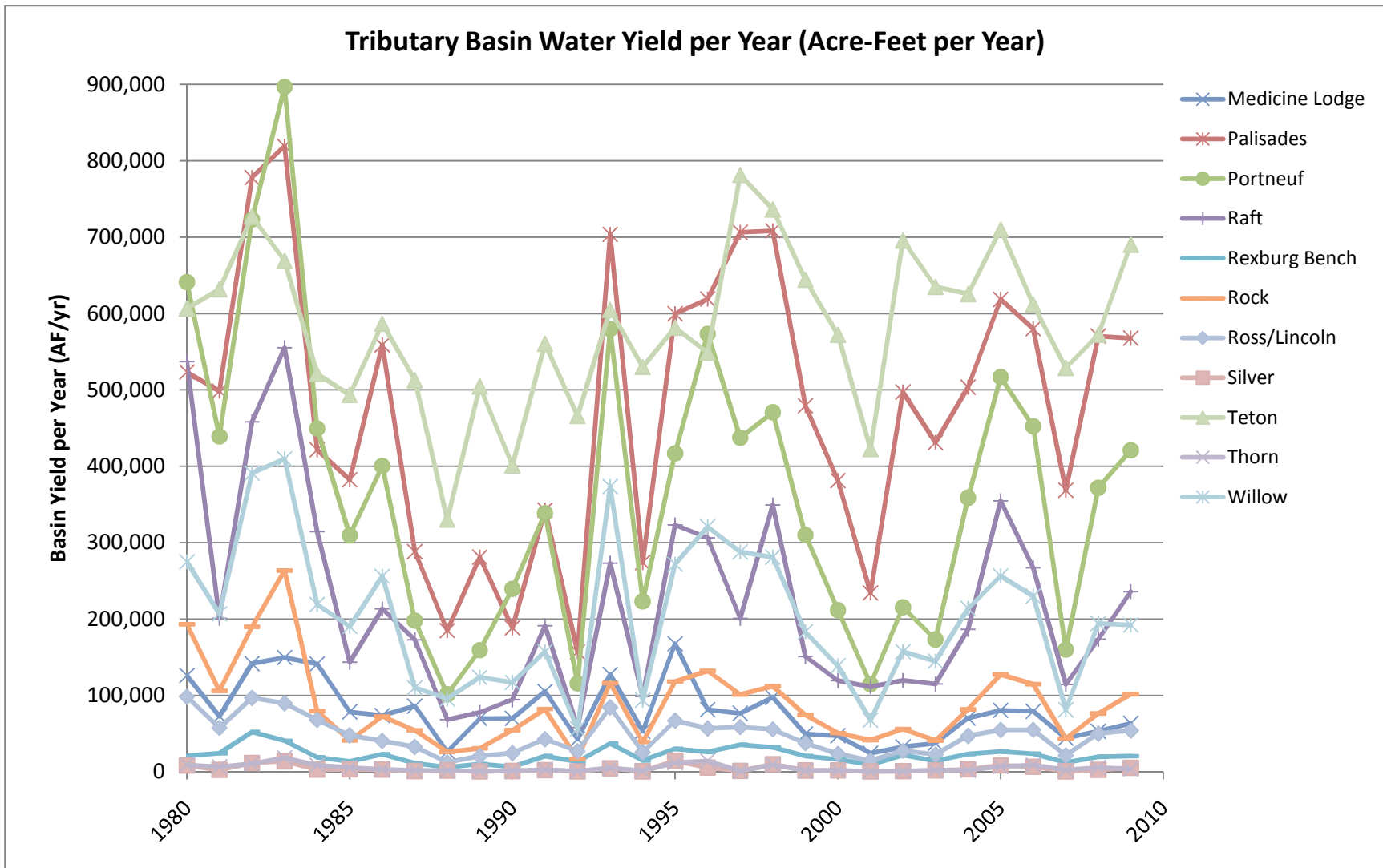
Figure 7b. Volume of water yield for tributary basins of the Eastern Snake River Plain aquifer. Water yield calculated using the Langbein method (Nace et al. 1961). Note that the vertical scale in this figure is smaller than the scale used in Figure 7a for the purpose of showing all basins clearly.
