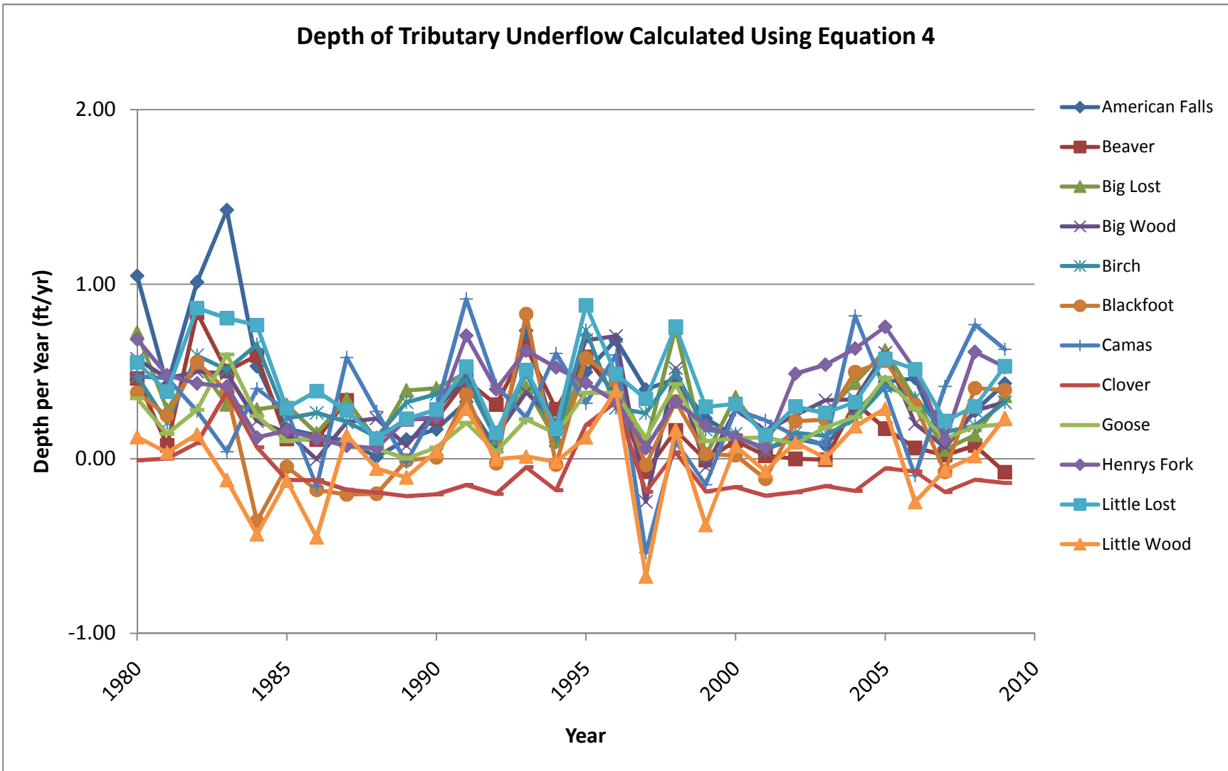
Figure 12a. Tributary underflow depths calculated using Equation 4.
