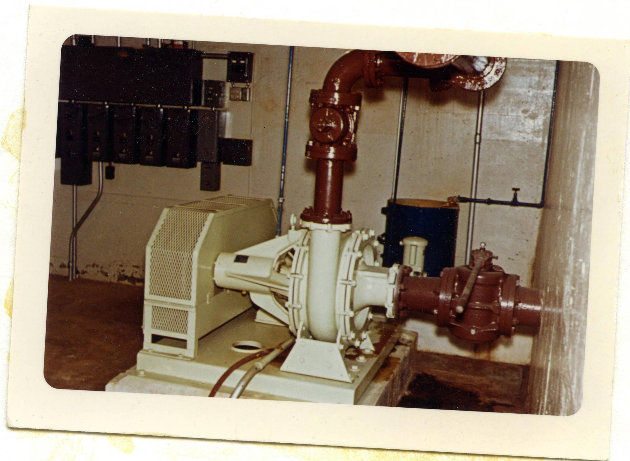
Secondary sludge pump
