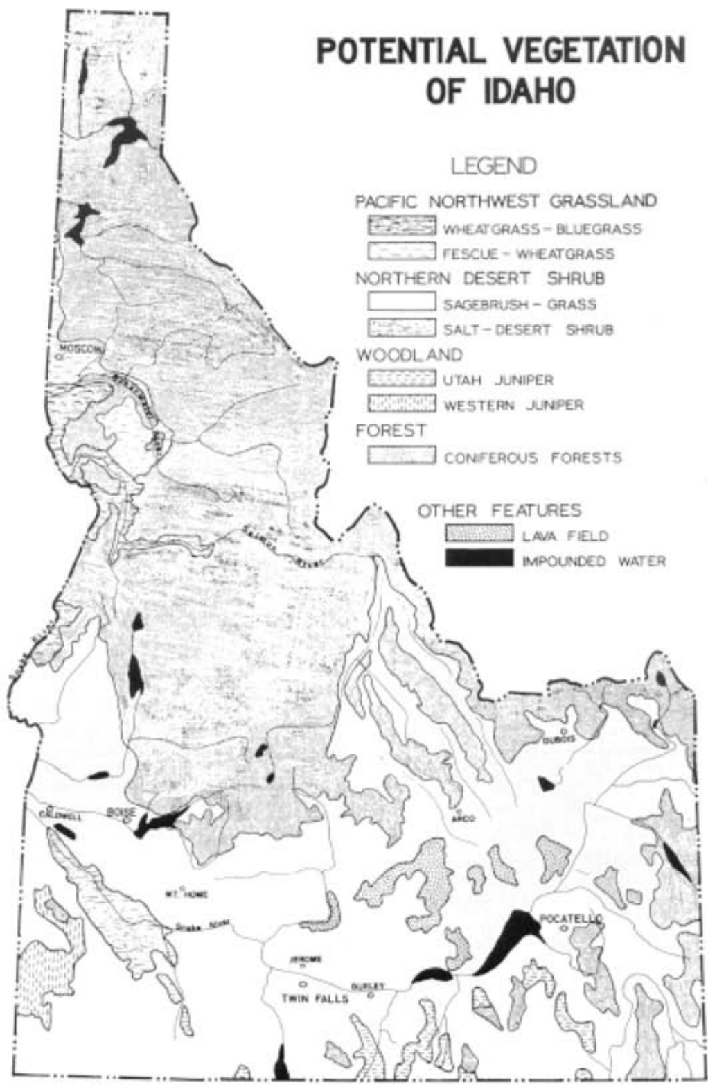
Fig. 4. Sketch map showing major potential vegetation types of Idaho. Revised from Kuchler (1964).
