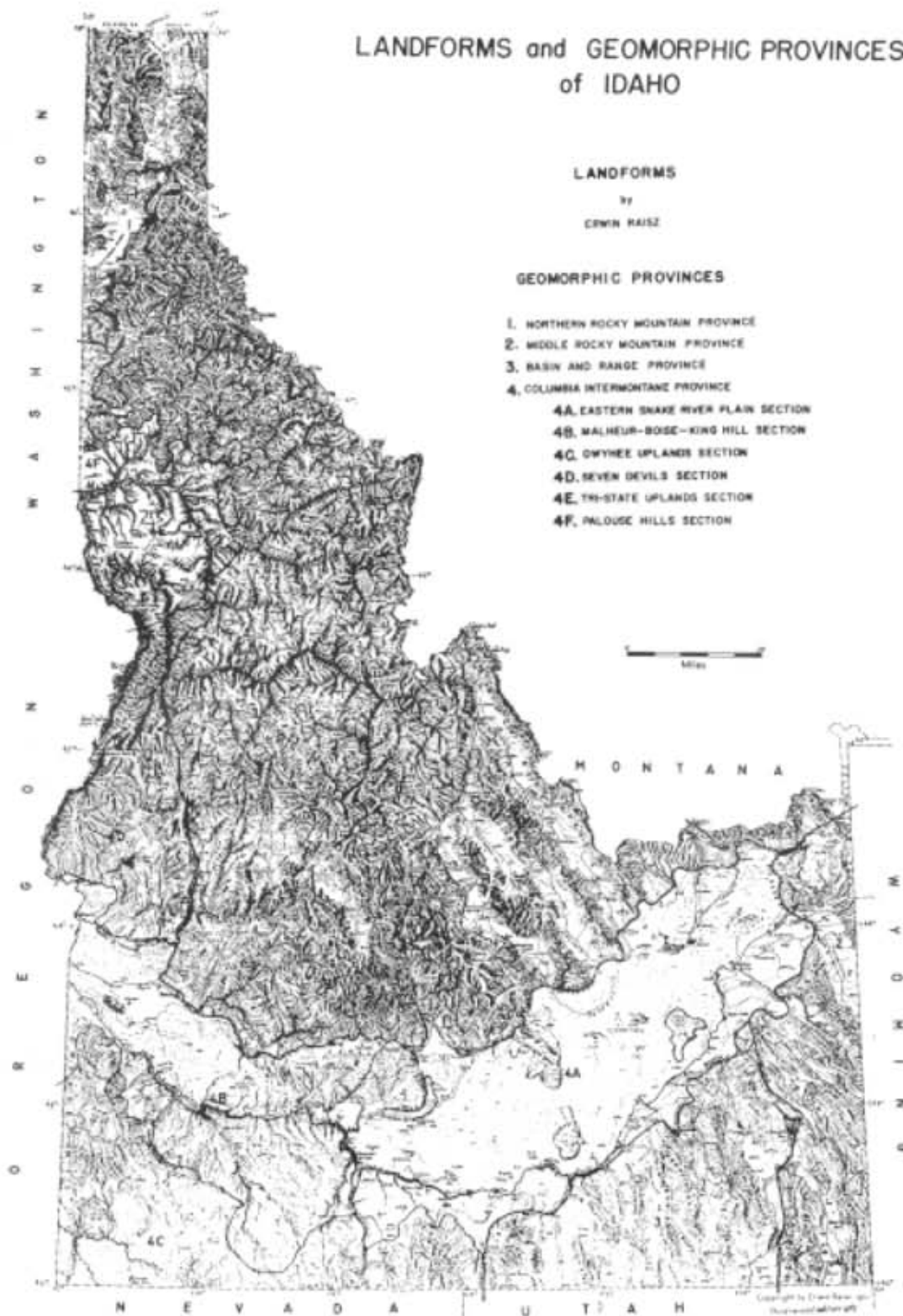
Fig. 5. Landforms and geomorphic provinces of Idaho. From Ross and Savage (1967).
