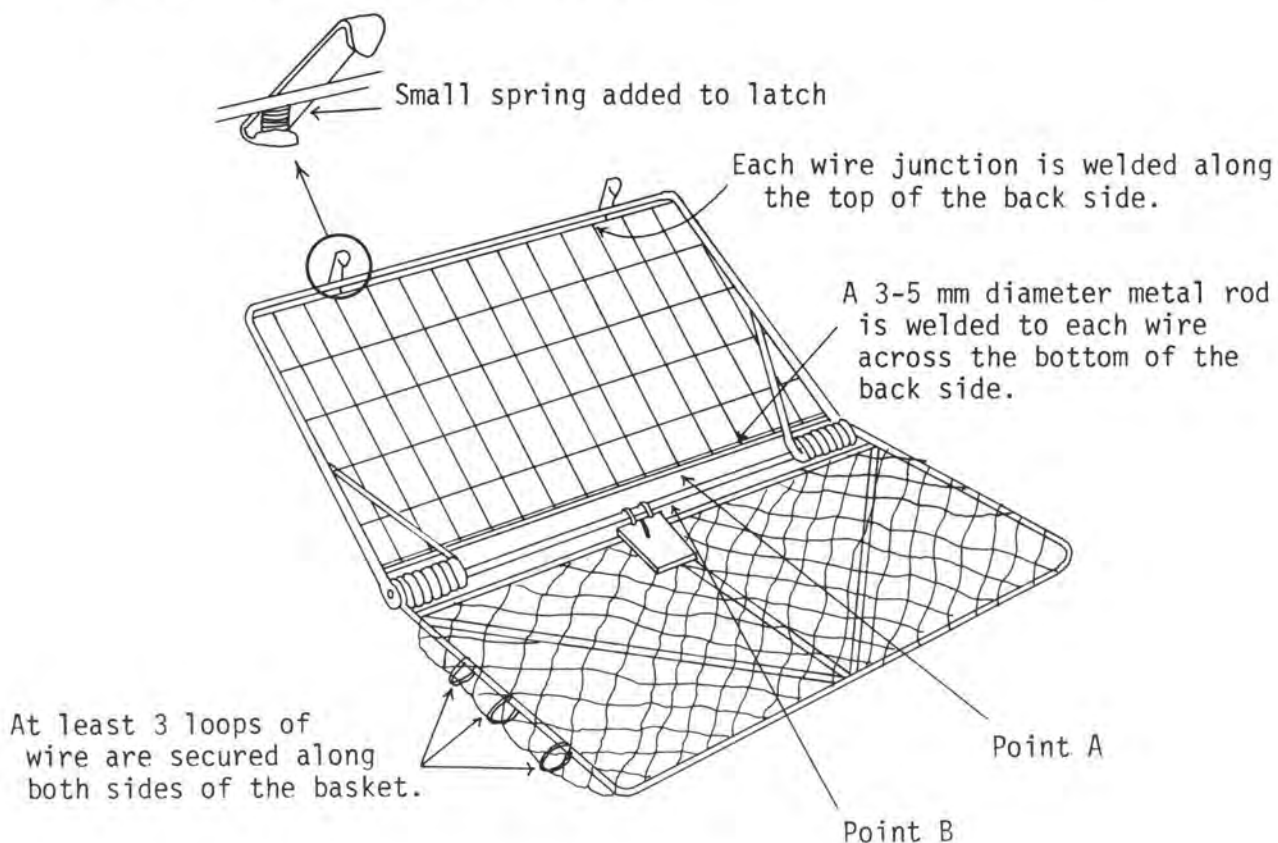
Figure 1. Modifications made to Hancock livetraps.
