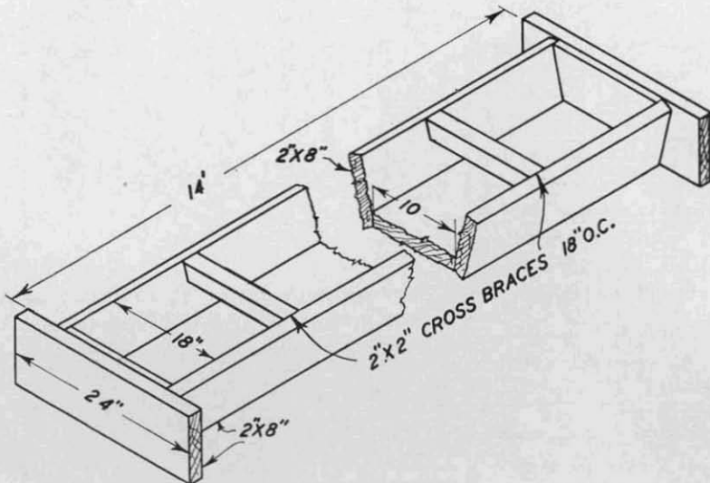
Fig. 17.—A satisfactory bevel box-type trough with reinforced ends.
