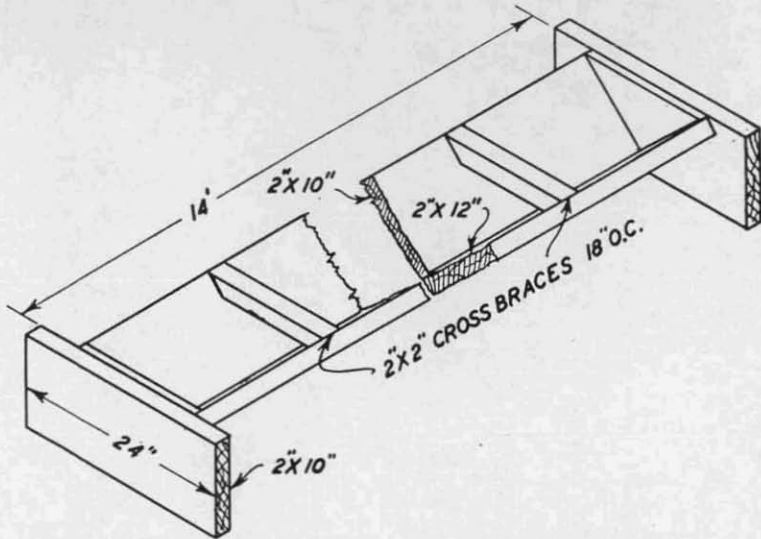
Fig. 16.—Conventional "V" type trough with reinforced ends.
