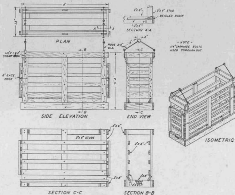
Fig. 19.—Lifting crate.
