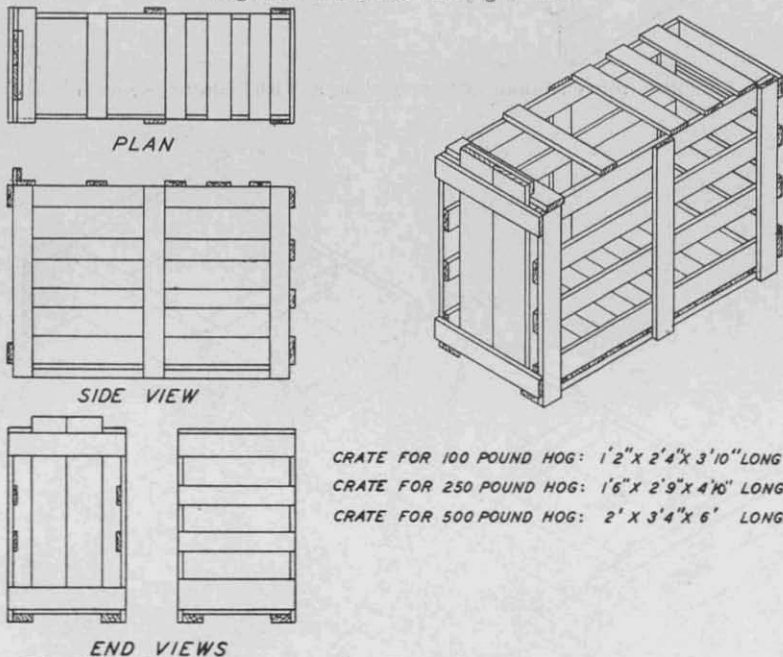
Fig. 15.—Shipping crate. The dimensions specified for the various weights are satisfactory under normal conditions.
