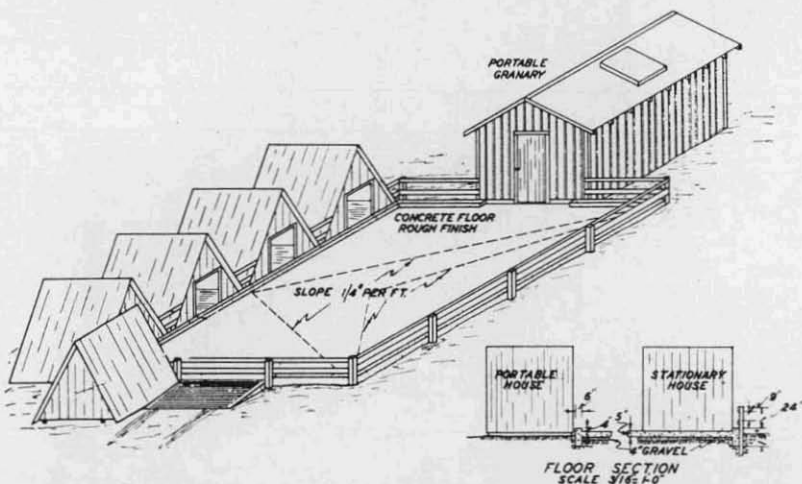
Fig. 21.—A good feeding floor can be used conveniently for early spring farrowing or as a centralized unit for wintering sows. Plans and specifications available through Department of Agricultural Engineering, University of Idaho.
