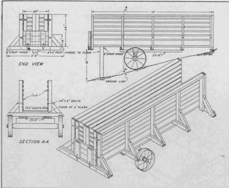
Fig. 14.—Portable loading chute.
