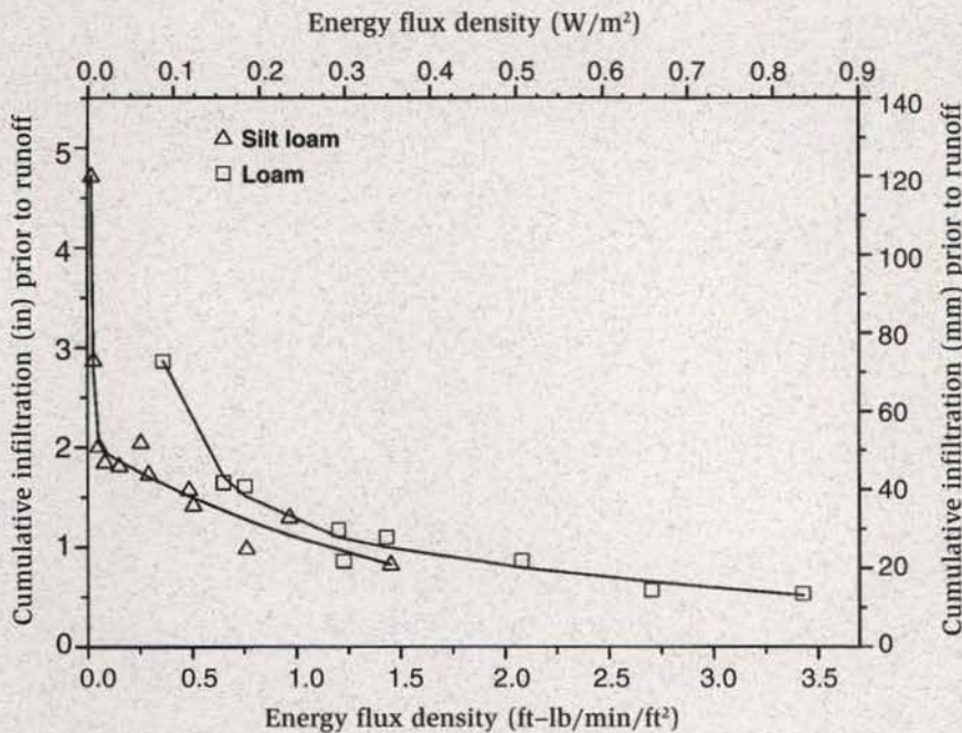
Figure 10. Infiltration rate reduction by energy density flux of sprinkler droplets for two soils. Adapted from Thompson and James (1985) and Mohammed and Kohl (1987).
