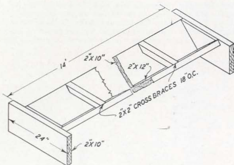
Fig. 20.—Standard V-type trough. Note reinforced ends and possibility for double nailing.
