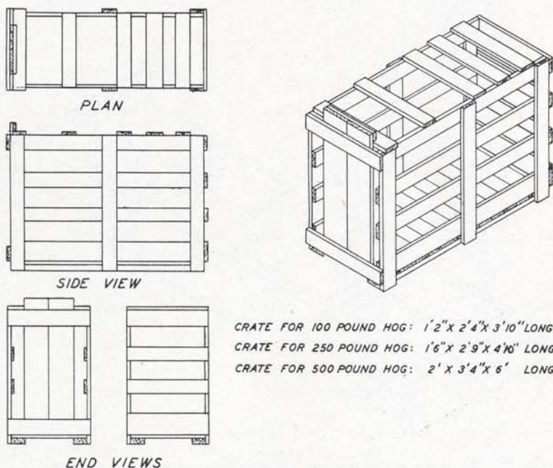
Fig. 19.—Shipping crate for hogs.
