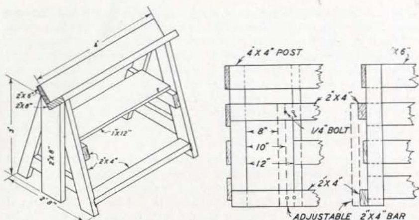
Fig. 13.—Convenient castrating trough.
