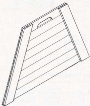
Fig. 25.—Hurdle "A" is made 3' long at the bottom and 1'6" long at the top. It is 2' high. Half inch ceiling material may be used for the body of the hurdle and \frac{1}{2} " by 3\frac{5}{8} " lumber for the ends. The handle should be made of 1" lumber.
