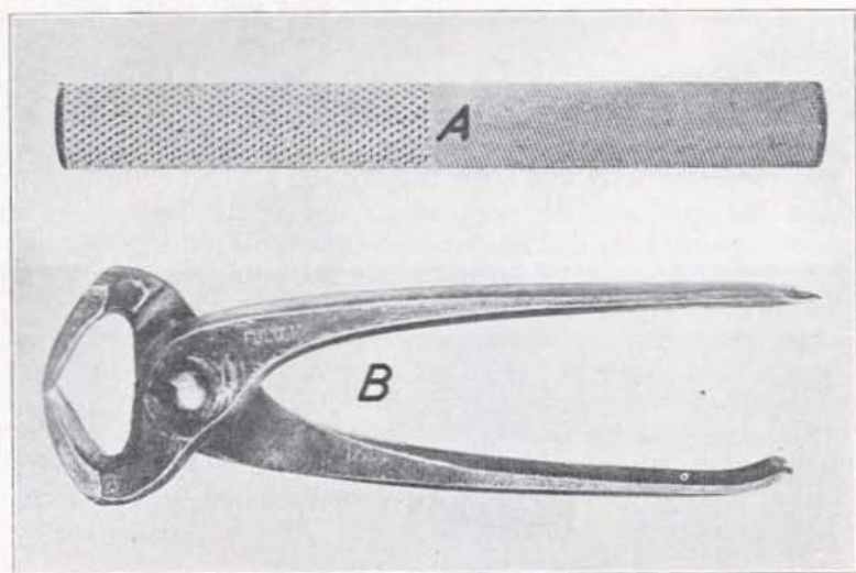
Fig. 23.—A—Eight-inch double rasp. B—Eight-inch nippers.
