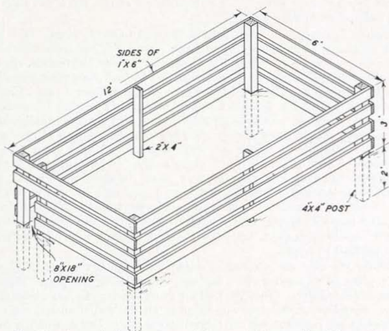
Fig. 14.—A practical pig creep, and (upper right) an adjustable opening.
