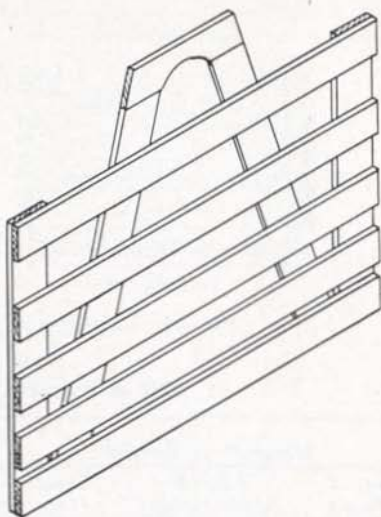
Fig. 26.—Hurdle "B" is made of \frac{1}{2} " by 3\frac{5}{8} " material. It is 3' long and 1'8" high. The hurdle length at the top is 10". The handle top of the hurdle is 8" above the body of the hurdle.
