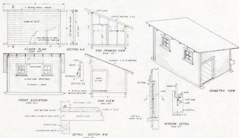
Fig. 18.—This one way roof field house affords more room than the "A" type house but it is a little more expensive to construct. Note ventilator in front. It is very satisfactory.
