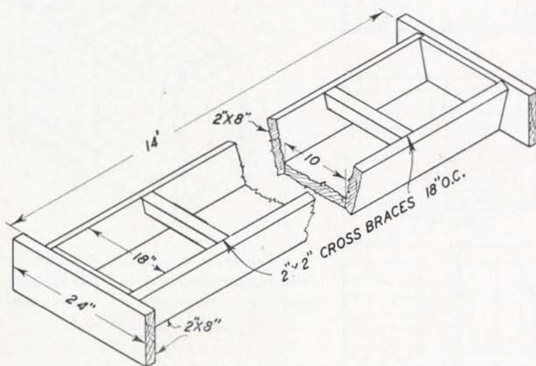
Fig. 21.—Beveled box type trough. Note reinforced ends and possibility for double nailing.
