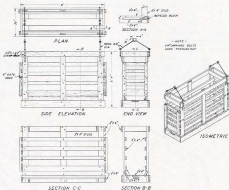
Fig. 24.—Lifting crate for use with large hogs.
