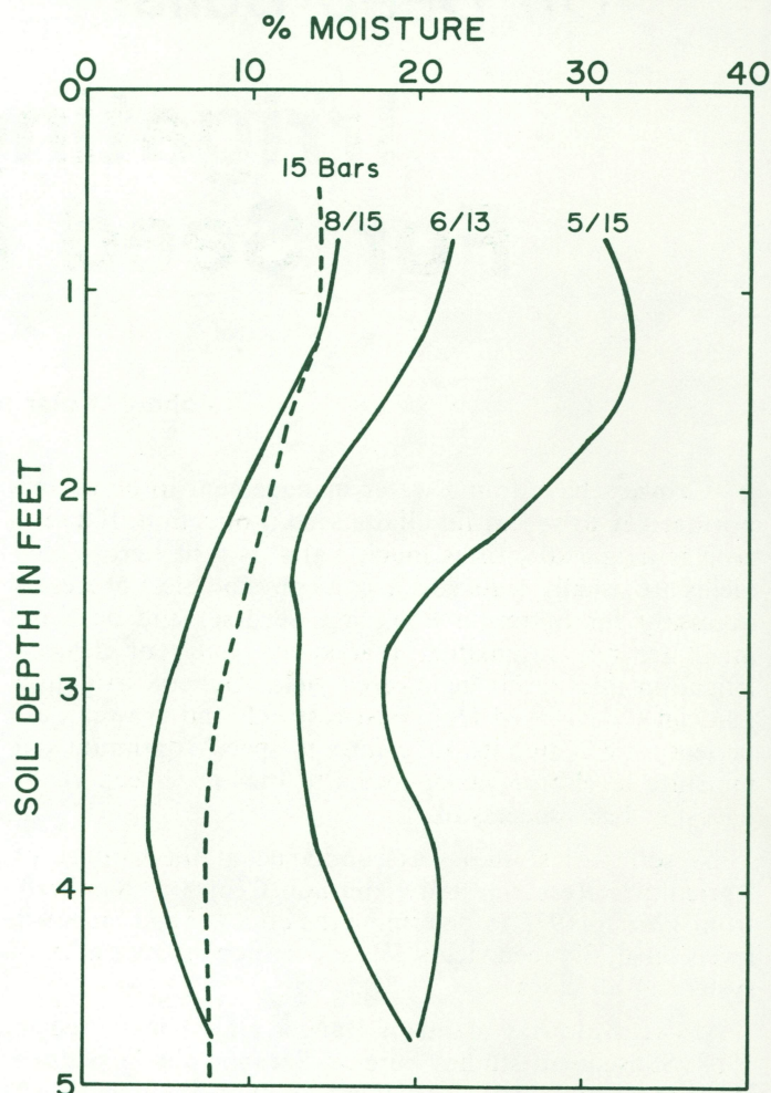
Fig. 1. Typical pattern of soil moisture extraction from the upper 5 feet of the soil profile by alfalfa grown under Treatment 5 at Kimberly, 1968.
