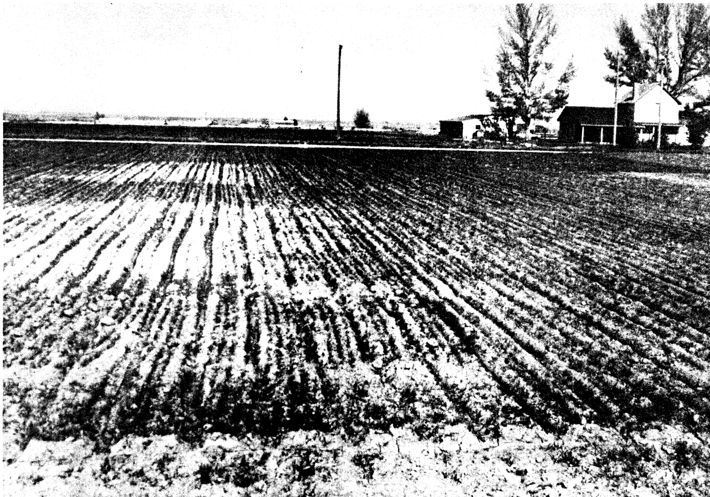
Fig. 4. White spots on the surface signal the high lime content and low organic matter of hardpan layers in southcentral Idaho's
