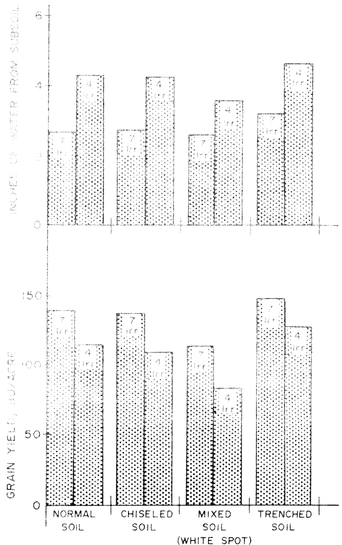
Fig. 3. Average corn yields and the amount of soil water removed below 2 feet after July 28 and November 3 in the fourth cropping season after deep tillage. The total water used by the crop ranged from 21 inches on lowest-yielding plots to 27 inches on highest-yielding plots.
