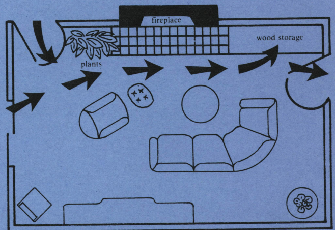
Location for the fireplace within a room is important. Drawing at top shows poor fireplace location; at bottom, good placement.
