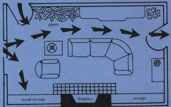
Location for the fireplace within a room is important. Drawing at top shows poor fireplace location; at bottom, good placement.
