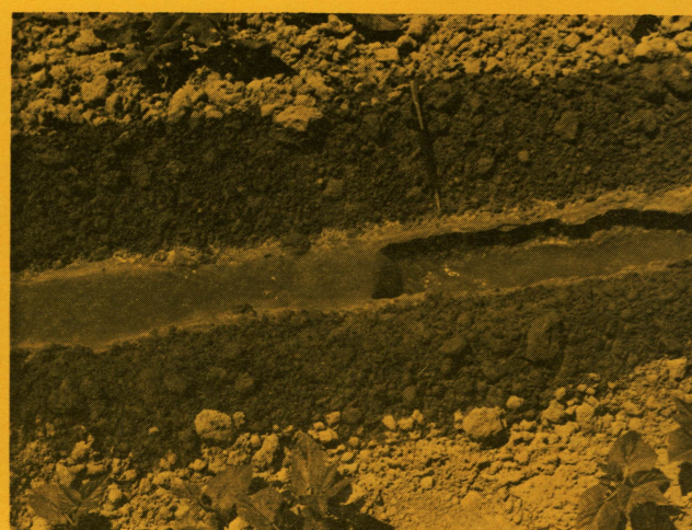
Fig. 4. Erosion near the end of a furrow. As the soil erodes, the water fall moves up the furrow.
