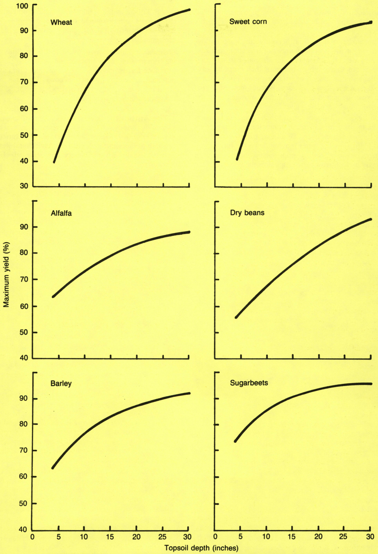
Fig. 2. Percent maximum yield at various topsoil depths for six crops grown on farmer's fields and experimental plots.
