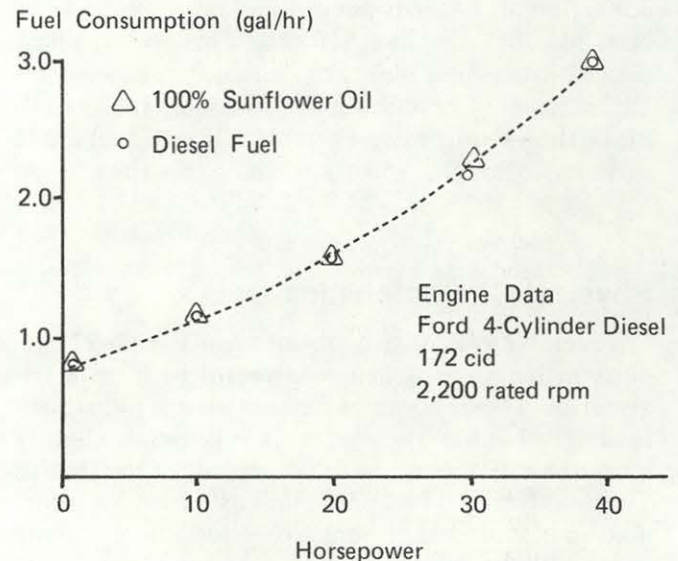
Fig. 1. Diesel engine performance using vegetable oils and vegetable oil-diesel mixtures as a fuel.
