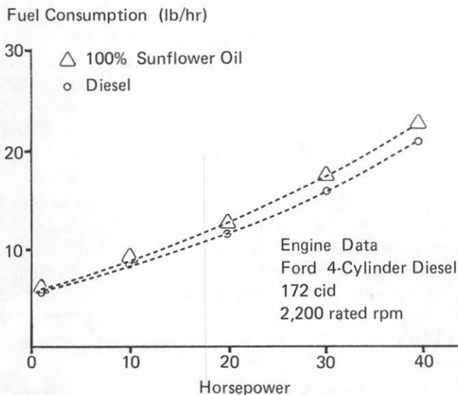
Fig. 2. Diesel engine performance of tests using vegetable oils and vegetable oil-diesel mixtures as a fuel.
